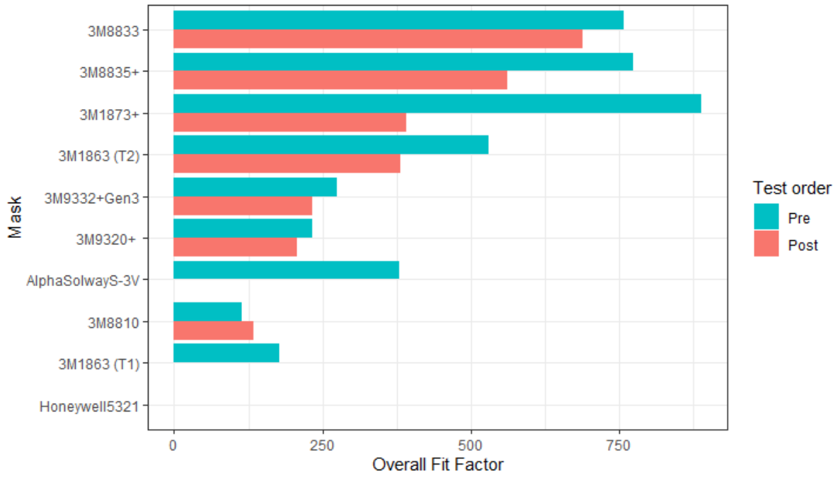
185 Figure 1: Overall fit factor of masks tested pre- and post- heat treatment (3M1863 was tested by two people)
