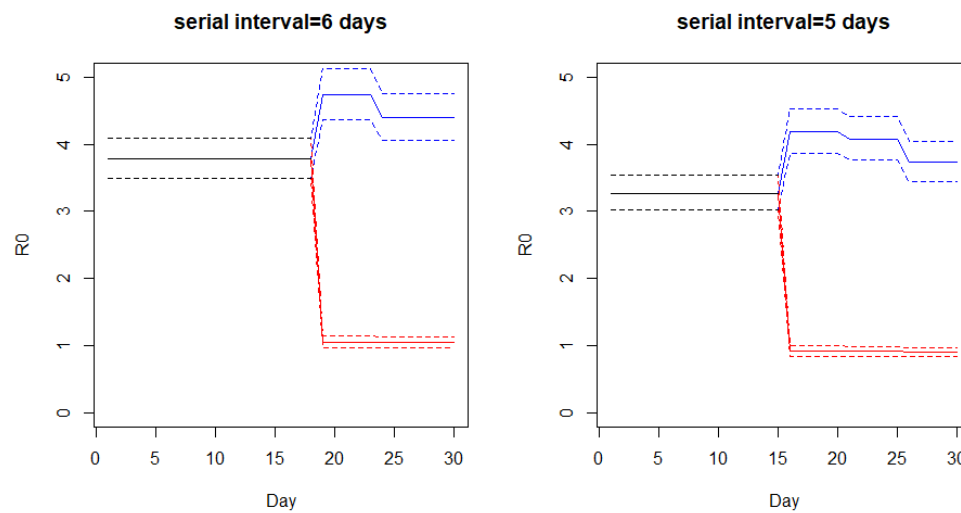
Figure 1: Time-dependent effective reproduction number R_0 (solid lines) of COVID-19 on board the Diamond Princess ship January 21 (day 1) to February 19 (day 30) and their 95% confidence intervals, assuming \tau = 5 and 6 days, r_p = 0.2 and aratio = 0.505 .
