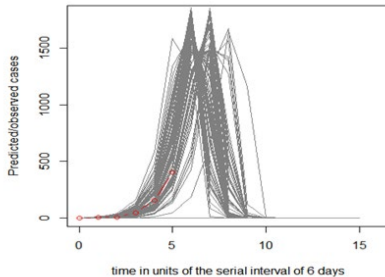
Figure 2: 100 stochastic simulations of the chain binomial model based on N = 3700 and estimated \beta = 3.78 , assuming no quarantine, infected cases removed, and extrapolation to 90 days, \tau = 6 , with the observed epidemic (red line).
