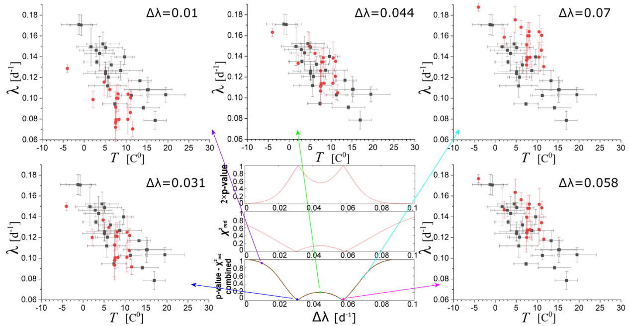
Figure 7. Fitting of datasets combined for US and Italian regions, with the latter's rates shifted by \Delta\lambda . The optimal fitting corresponds to shifts \Delta\lambda \sim 0.031 and \sim 0.058 , for which the reduced chi-square is \sim 1 , the p -value of the extremes is \sim 0.5 , and the combined measure \sim 0 .
