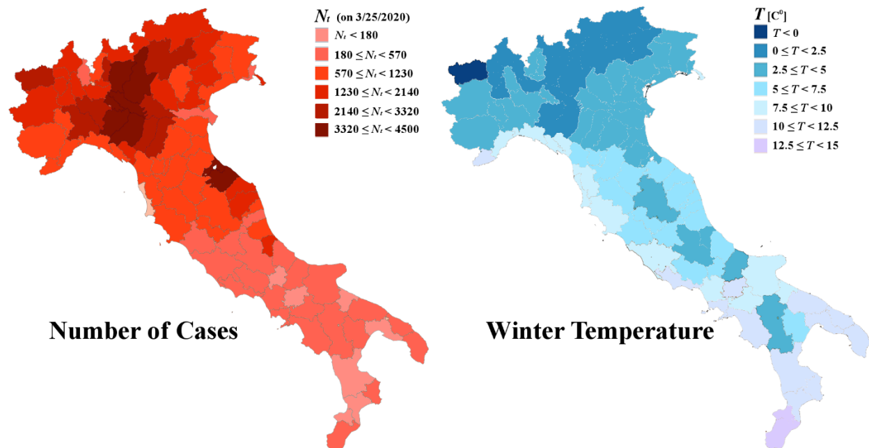
Figure 2. Regional distribution of infected cases N_i by 3/25/2020 (left), and average winter temperature T in mainland Italy (right).
