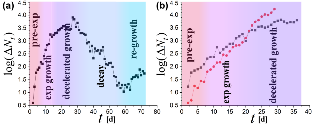
Figure 1. Evolution of new cases infected by COVID-19 (on linear-log scale) for mainland China (left) and US & Italy (right); phases (color-coded): pre-exponential (pre-exp), exponential (exp) growth, decelerated growth, decay (or decline), and possibly, a re-growth. Day t=1 corresponds to 1/15/2020 for China, 2/20/2020 for Italy, 2/27/2020 for US. Evolution in China cases follows the whole growth-decay cycle, and a new re-growth phase. Italian cases are characterized by a milder exponential rate, entered the phase of decelerated growth on March 12. US suffers with a larger exponential rate, and it is not clear whether has entered the decelerated growth phase. The exponential growth rate for China rose as high as \lambda=0.169\pm 0.017 , while for Italy and US the rates were \lambda=0.090\pm 0.004 and 0.121\pm 0.003 , respectively (with correlation coefficient > 0.99 ).
