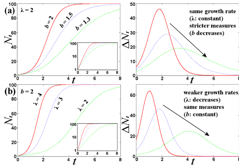
Figure 3. Plots of total N_t and new \Delta N_t infected cases according to model (1), showing the flattening of the spread curve with the interplay of (a) stricter measures (decreasing b ), or (b) weaker rates (decreasing \lambda ). (Input panels show graphs on semi-log scale.)
