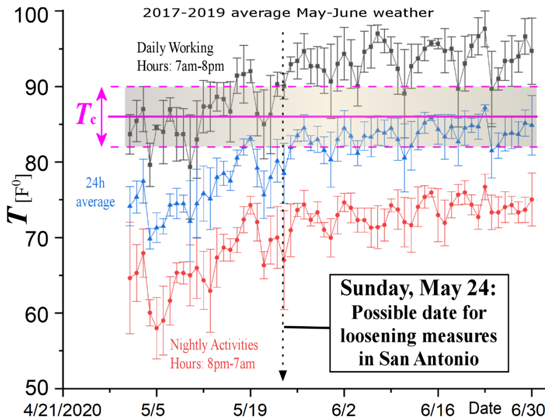
Figure 10. According to the statistically confident relationship between exponential growth rate of infected cases shown in Fig 8, the critical temperature, which eliminates the exponential growth, and thus the COVID-19 spread, is T_c = 86.1 \pm 4.3 \text{ F}^\circ . The plot shows also the May-June daily, nightly, and 24h-averaged environmental temperatures in San Antonio, Texas, averaged over the last three years. The daily average temperatures will be clearly above the estimated T_c threshold in the second half of May; thus, the plot suggests a possible date for loosening the strict measures in San Antonio, that is, May 24.
