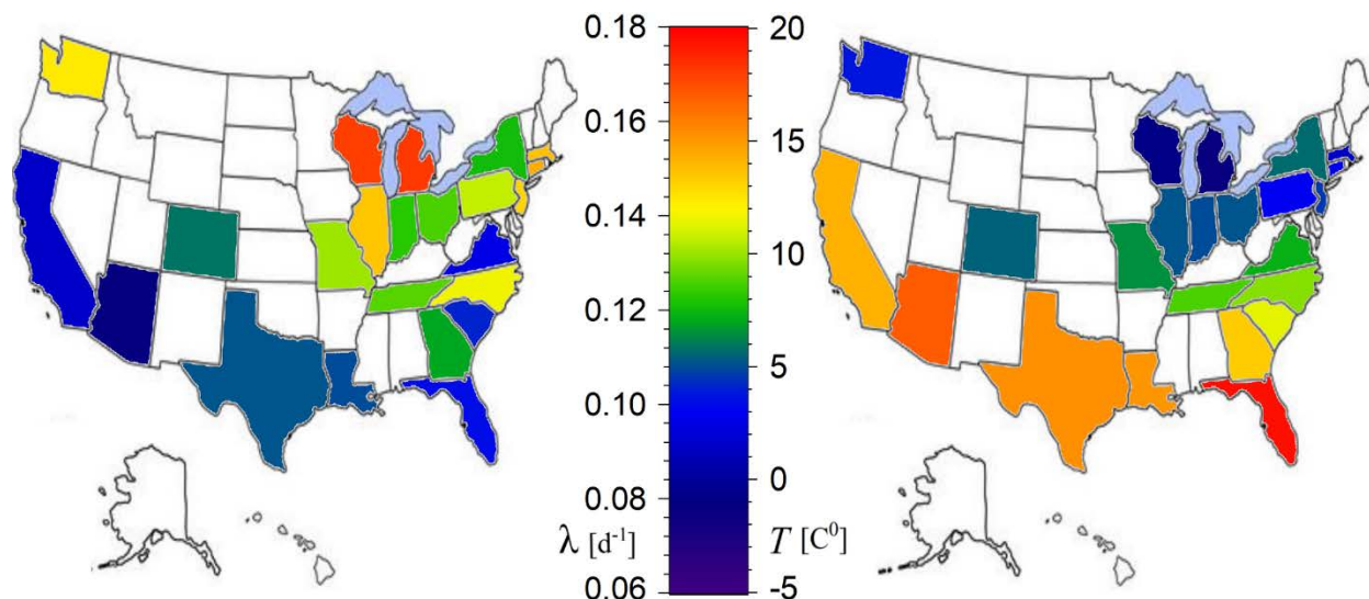
Figure 9. Anti-correlation between the spatial distributions of the exponential growth rates of the infected cases (left) and the average environmental temperature (right).
