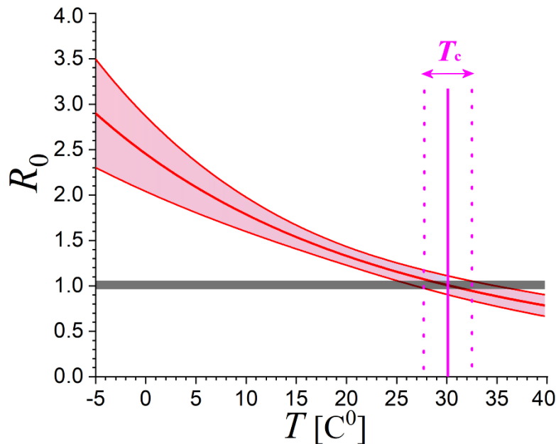
Figure 8. Relationship of the reproduction number R_0 and its uncertainty with environmental temperature T . According to this, new affected cases cease ( R_0=1 ) when temperature climbs to T_c \sim 30 C 0 or ( \sim 86 F 0 ).
