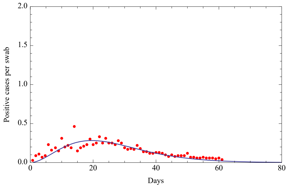
Fig. 2a Fit of the ratio of daily positive cases per swab obtained with a function of the type of the Planck's black body law with two parameters, with the exponent of the time variable t equal to 3 as in the Planck's law. The beginning date is February 25. Root Mean Square of the residuals is 0.050
