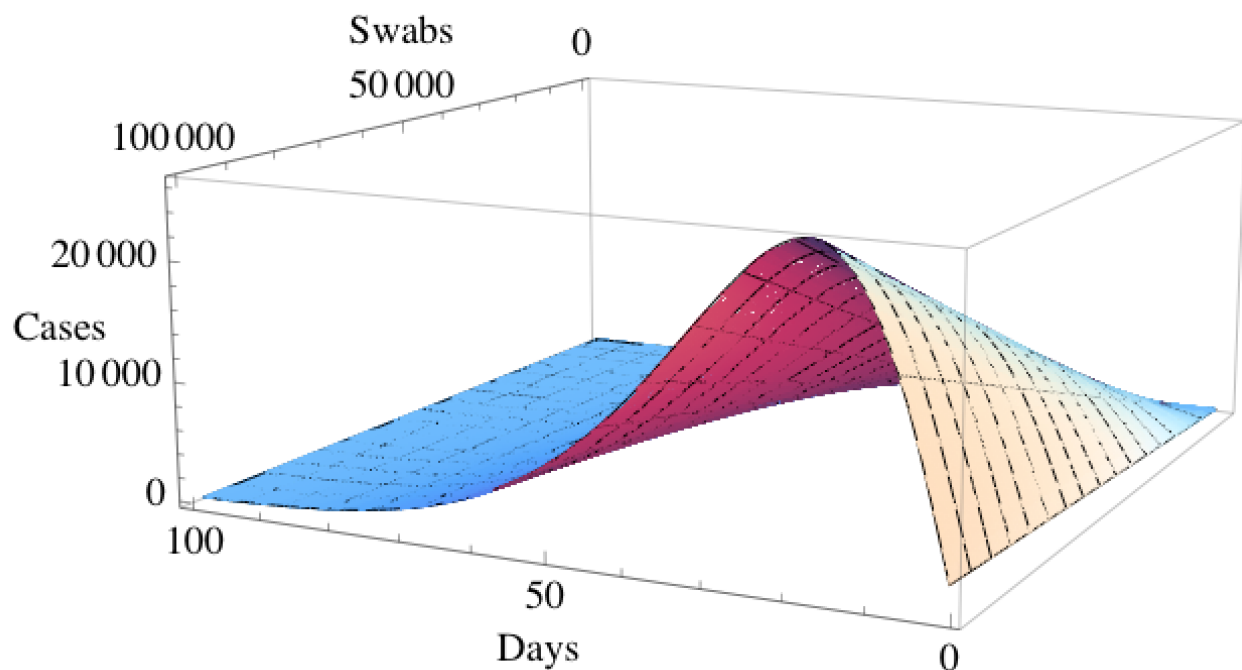
Fig 3. Representation in 3D of the number of daily cases as a function of the number of daily swabs (from 0 to 100000) and of the day, from February 25, for a distribution of the type of Planck's law with three parameters used to describe the positive cases per swab.
