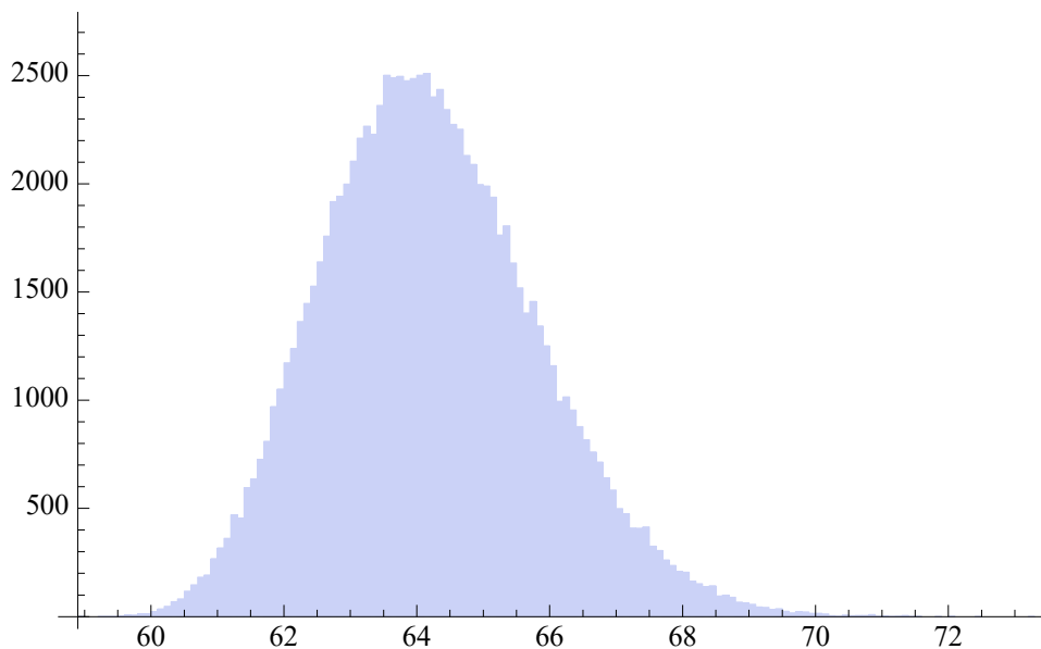
Fig. 7 Result of 100000 simulations using the 20 Italian regions for a possible estimate of the uncertainty in the date of a substantial reduction in the number of daily positive cases.
