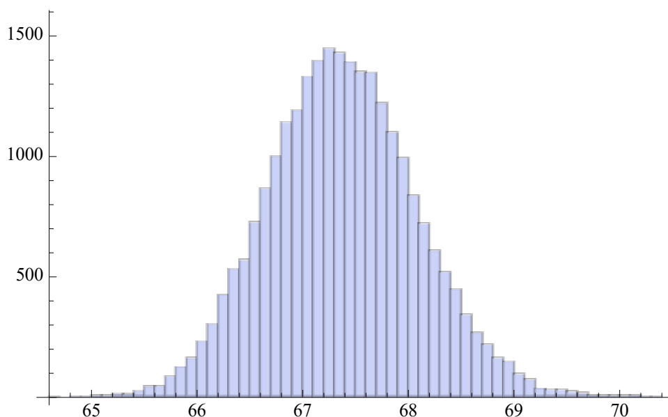
Fig. 5. Histogram of the 25000 runs of the Monte Carlo simulation for Italy: frequencies versus the day in which a substantial reduction in the number of daily cases occurs.
