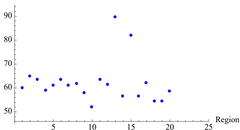
Fig. 6. Dates of a substantial reduction in the number of daily diagnosed positive cases for each of the 20 Italian regions. The 1-sigma standard deviation is about 9 days.
