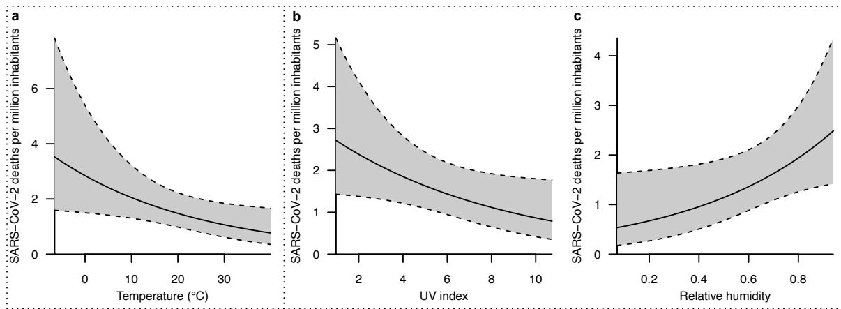
Figure 1. Climatic factors influencing the mortality rate during the COVID-19 outbreak (calculated per million inhabitants). A) effect of temperature (in degrees Celsius), B) effect of UV-index, C) effect of relative humidity. Because temperature and UV-index are highly correlated (see methods), these two variables were analysed separately in two distinct models. The influence of humidity is taken from the UV-based model.
