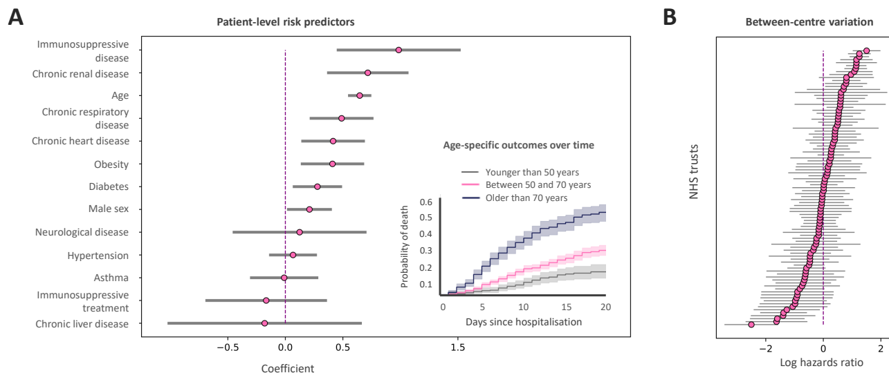
Figure 1: Panel (A) Fixed effects (log hazard ratio) estimates for CHES predictors. The inset shows mortality probability over time for young, intermediate and older age groups. Panel (B) random effects (log hazard ratio) showing between centres variation. (95% CIs).
