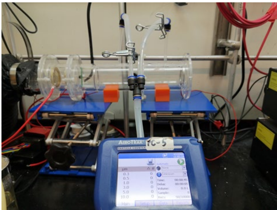
Supplementary Figure 2: Image of ambient particulate matter air ducts used in MIT testing of N95 masks. Note that this is a destructive test in which the N95 mask is cut prior to introduction into the testing chamber.
