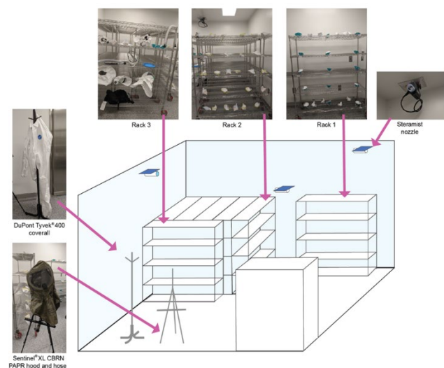
Figure 1: Diagram illustrating the testing set-up for SteraMist sterilization, with accompanying representative images. The chamber has an overall volume of ~80 m 3 .
