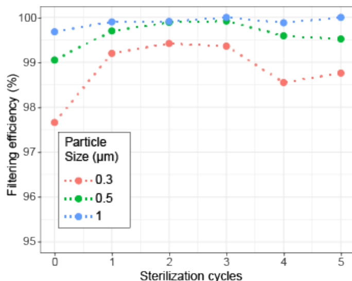
Figure 2: Ambient particulate matter filtration data for 3M 1860 masks over five SteraMist sterilization cycles. Each mask was tested in a university laboratory for filtration efficiency at three particle sizes (0.3, 0.5 and 1.0 \mu\text{m} ). Two masks were tested at two cycles and showed similar filtration efficiency; one mask is shown here.
