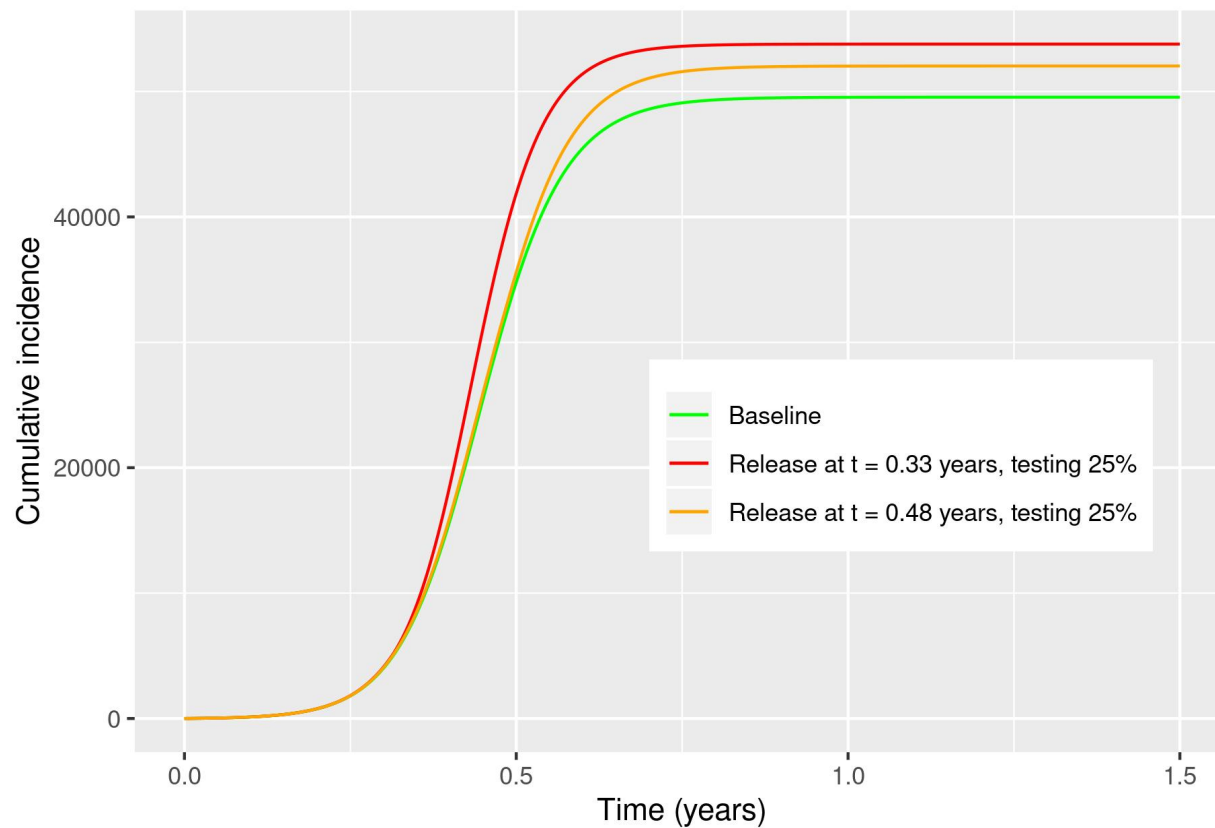
Figure 10: Cumulative incidence for a example population of 100k people. NPI are assumed in place, and release is assumed at time of testing. Asymptomatics are 25% of the infectious population.
