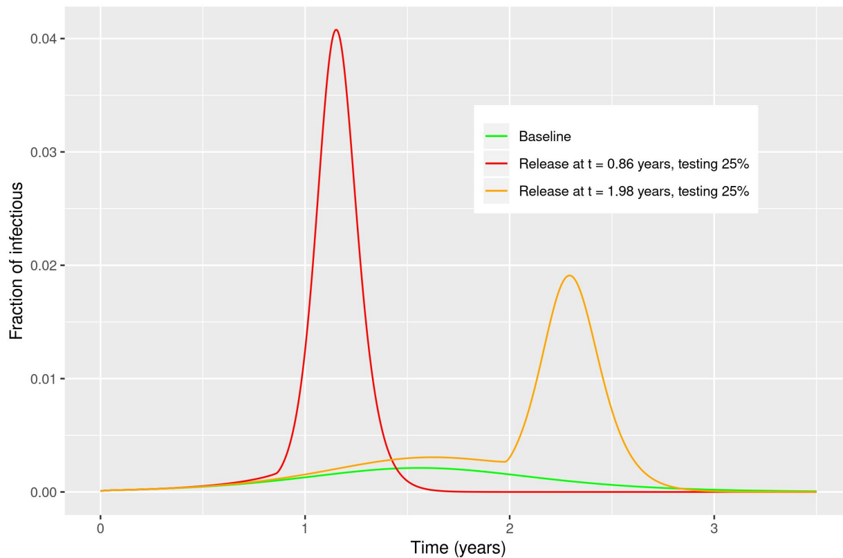
Figure 11: Effect of testing and social distancing, at different times, when asymptomatics are 85% of the infectious population. If 25% of the population is tested, a strong resurgence of the epidemic is observed if release of NPI occurs before the epidemic peak. Testing at or after the epidemic peak results in a strong secondary peak of infection.
