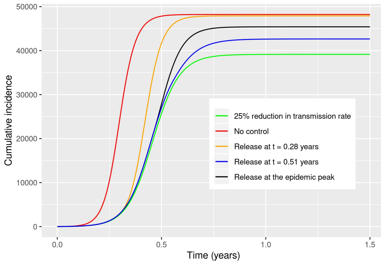
Figure 3: Cumulative incidence for an example population of 100k , with release of control at different times. Asymptomatics make for 85% of the infectious population. 25% reduction of transmission is achieved by reducing the asymptomatic transmission rate.
