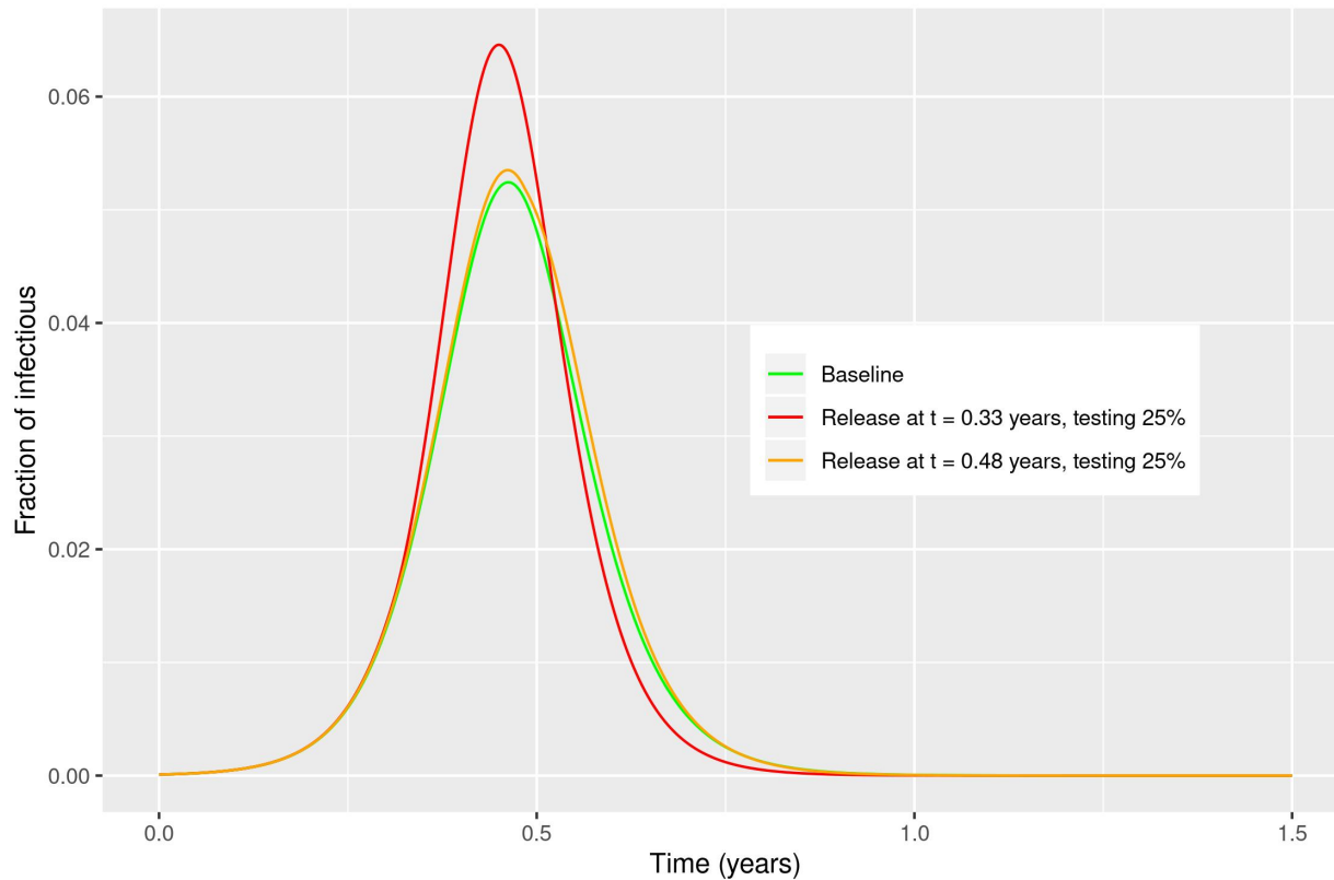
Figure 9: Effect of testing and social distancing, at different times, when asymptomatics are 25% of the infectious population. If 25% of the population is tested, a strong resurgence of the epidemic is observed if release of NPI occurs before the epidemic peak. On the other hand, testing at or after the epidemic peak results in a negligible difference between full control and release of control.
