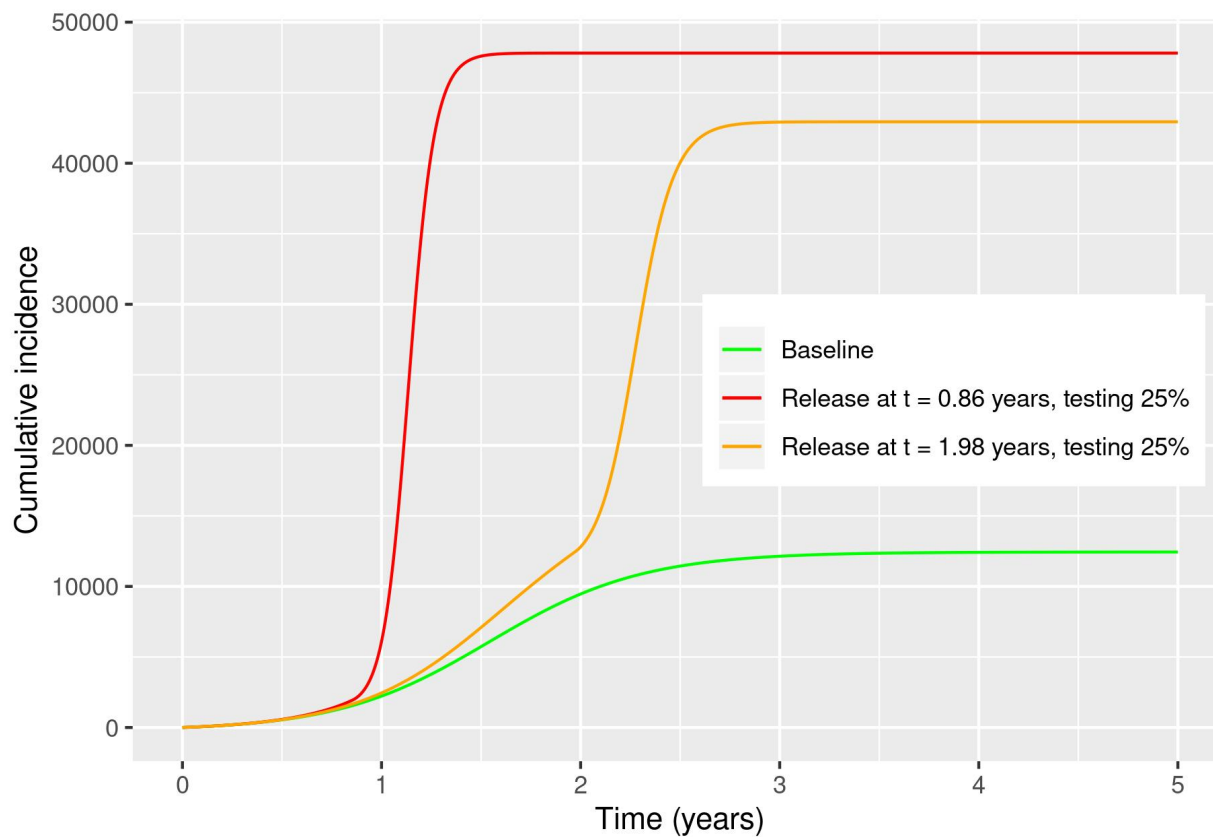
Figure 12: Cumulative incidence for a example population of 100k people. NPI are assumed in place, and release is assumed at time of testing. Asymptomatics are 85% of the infectious population.
