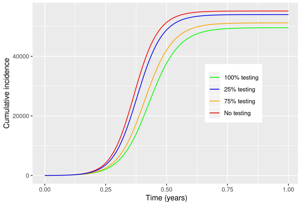
Figure 6: Cumulative incidence for a example population of 100k people, for various fractions of the asymptomatic population tested. Asymptomatics are 25% of the infectious population.
