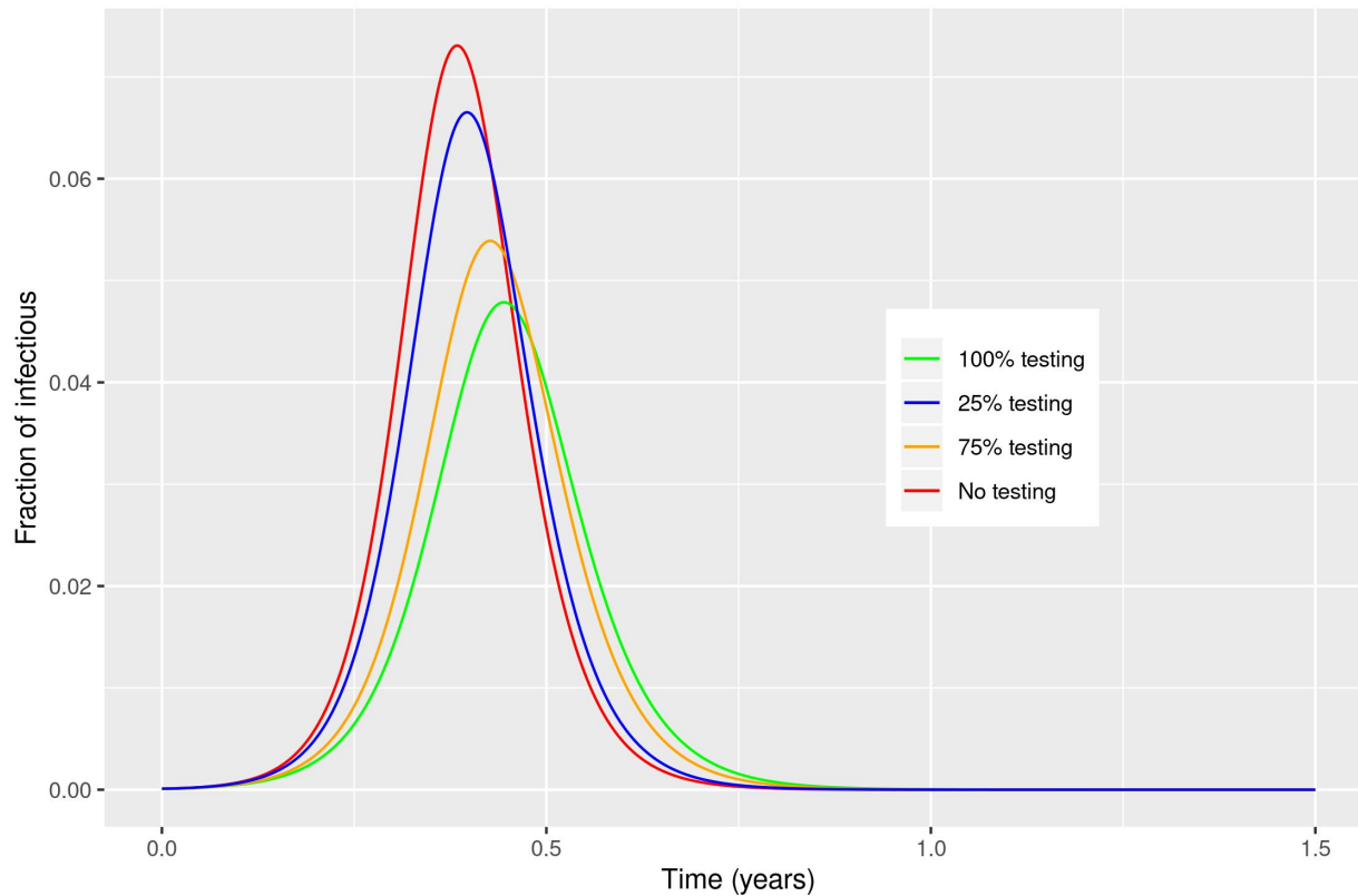
Figure 5: Effect of testing a fraction of the asymptomatic population as soon as the first case of infection is reported, in the absence of additional NPI. The asymptomatic make for 25% of all infectious cases. While a secondary peak is not observed, testing asymptomatics is predicted to reduce the intensity of the epidemic peak.
