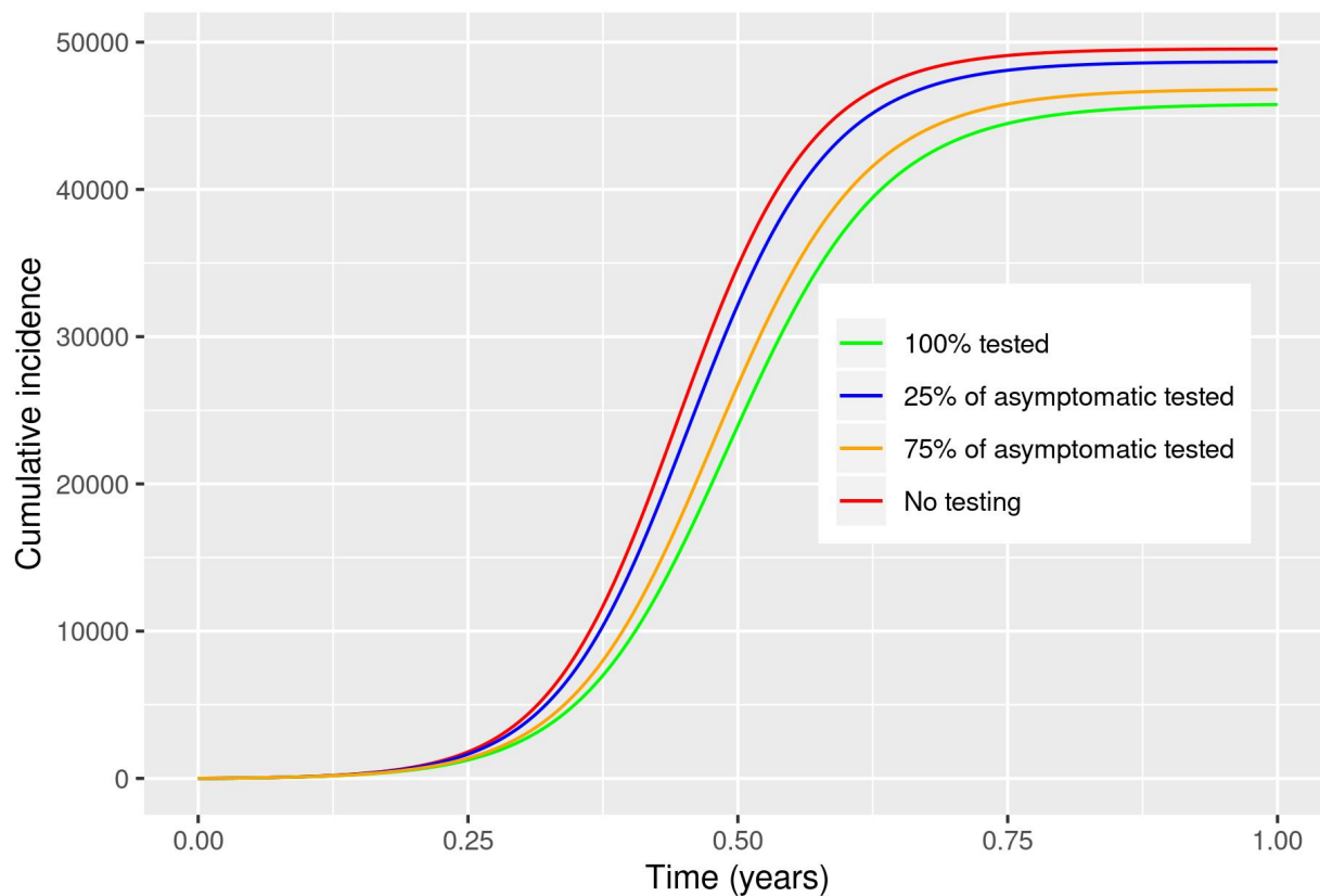
Figure 8: Cumulative incidence for a example population of 100k people, for various fractions of the asymptomatic population tested. Asymptomatics are 85% of the infectious population
