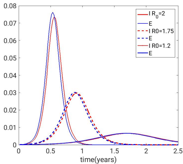
Figure 13: Exposed (blue) and infected (red) for R_0 = 2, 1.75 , and 1.2 . R_0 = 1.75 corresponds to quarantining 1 in 4 people from the population. That is reflected in a 25 percent reduction in the contact rates. Other parameters where rates are in years: \mu = 0.02, \mu_d = 0.035, \alpha = \gamma = 36.5 . \beta is adjusted to get the appropriate value of R_0 .
