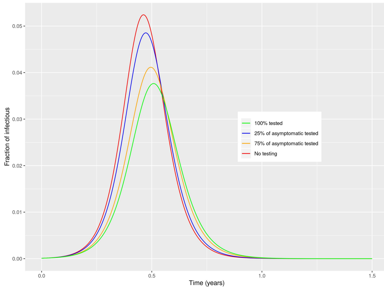
Figure 7: Effect of testing a fraction of the asymptomatic population as soon as the first case of infection is reported, in the absence of additional NPI. The asymptomatics make for 85% of all infectious cases. While a secondary peak is not observed, testing asymptomatics is predicted to reduce the intensity of the epidemic peak.
