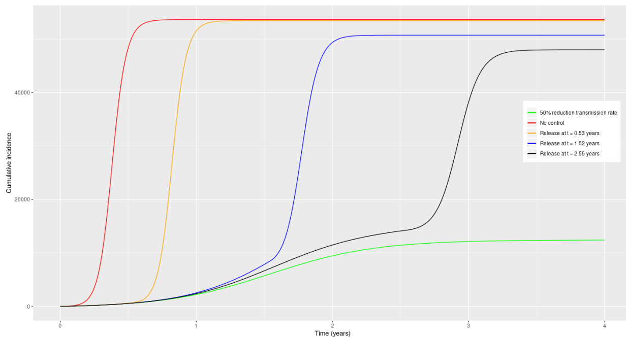
Figure 4: Cumulative incidence for an example population of 100k , with release of control at different times. Asymptomatics make for 85% of the infectious population. 50% reduction of transmission is achieved by reducing the asymptomatic transmission rate.
