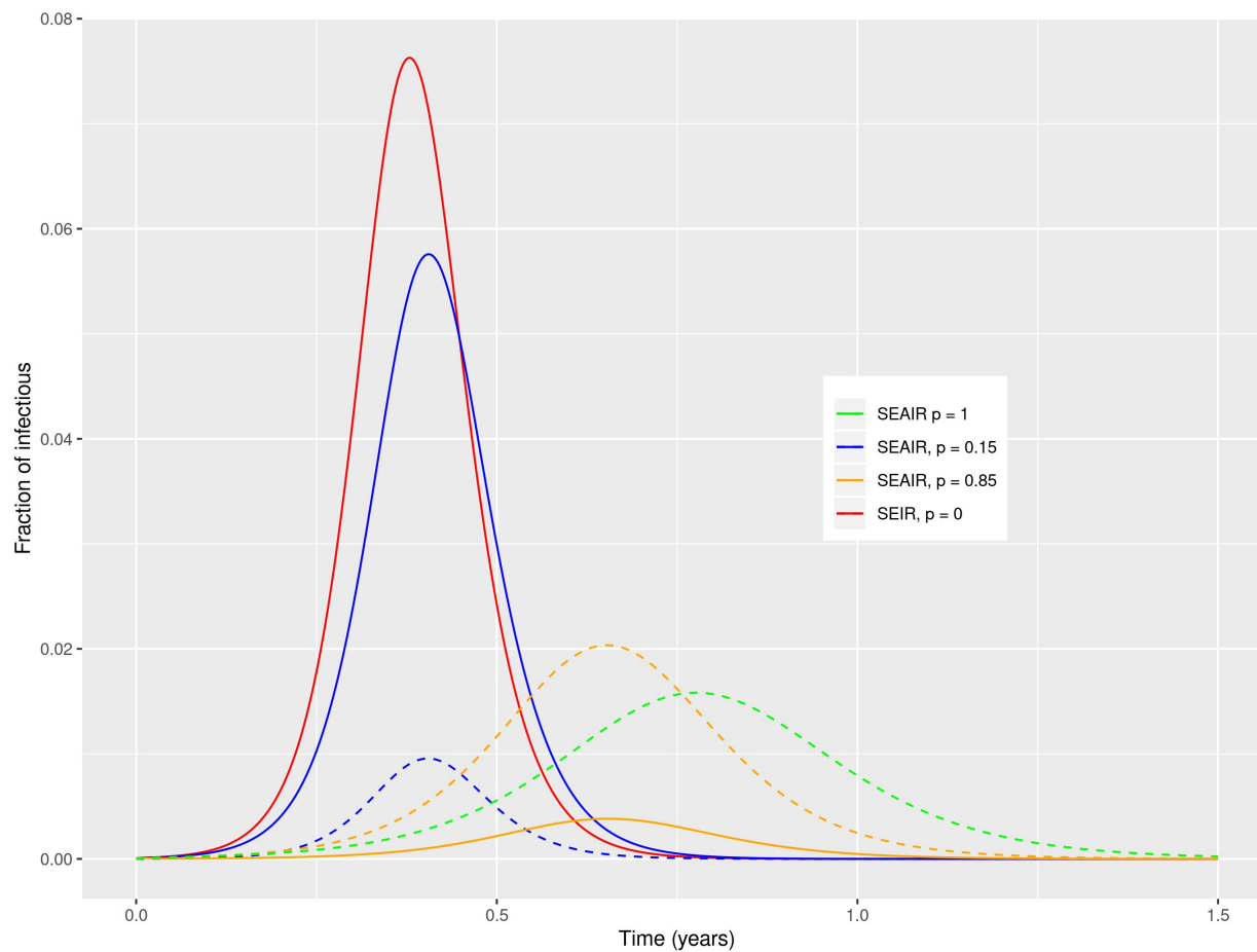
Figure 16: Comparison between SEIR and SEAIR for various fractions of the asymptomatic population, p . The solid lines represent the symptomatic infectious class, I . The dashed lines are the asymptomatic infectious, A . We observe that not including asymptomatic incorrectly estimates both size and timing of the infectious peak.
