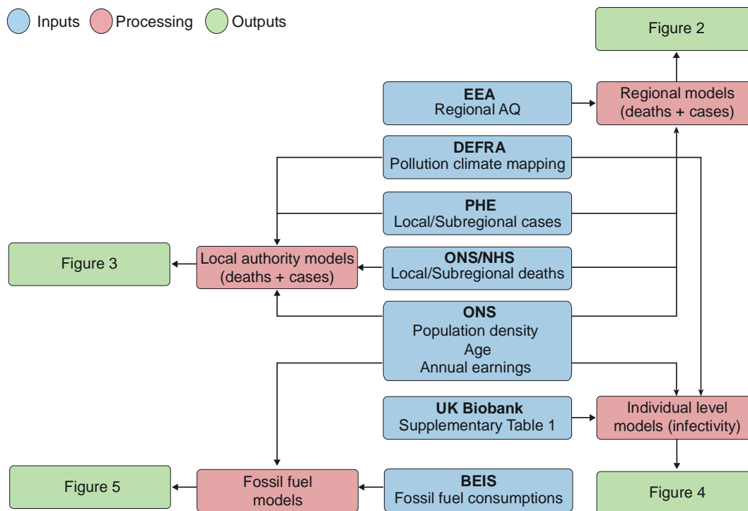
Figure 1. Analysis workflow.
