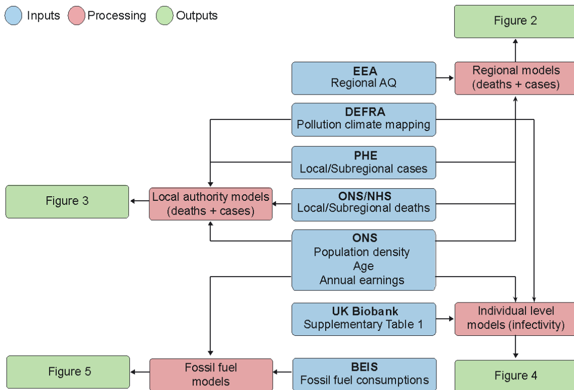
Figure 1. Analysis workflow.
