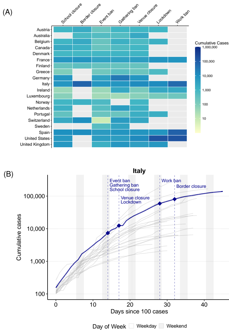
Fig. 1 (A) Heatmap showing the cumulative number of documented COVID-19 cases for each country until a non-pharmaceutical intervention is implemented. By reporting the cumulative number of cases, the heatmap highlights the ordering of health-policy measures within countries. If an NPI is not implemented by a country, it is colored gray. (B) Temporal development of cumulative cases for Italy, starting from 100 cases, with additional vertical lines referring to the points at which non-pharmaceutical interventions are enforced. The temporal development of cumulative cases for the other countries in the data is indicated by gray lines.
