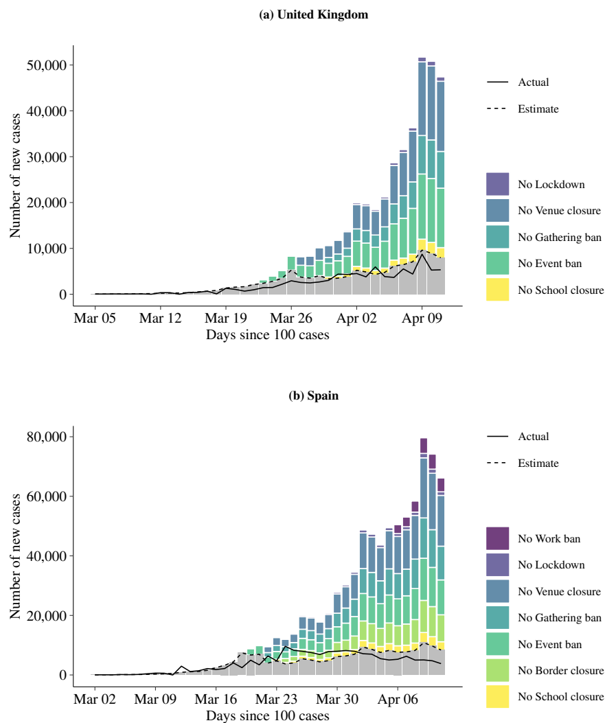
Fig. 3 Shown is the hypothetical effect of NPIs on the number of new cases. Specifically, it is illustrated how the mean estimated number of new cases would have changed if NPIs had not been imposed (stacked bars). The solid line refers to the actual and the dashed line to the estimated number of new cases based on the NPIs the corresponding country imposed. The NPIs are shown for the time period in which they were in force while considering that their effect is subject to a time delay of 7 days.
