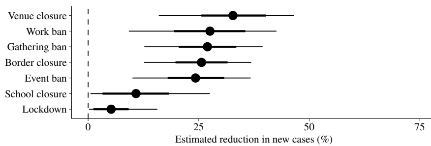
Fig. 2 Shown is the estimated reduction (mean as circle) in the number of new cases (in %) for each non-pharmaceutical intervention (NPI). The 80% and 95% credible intervals are indicated by thick and thin lines, respectively.
