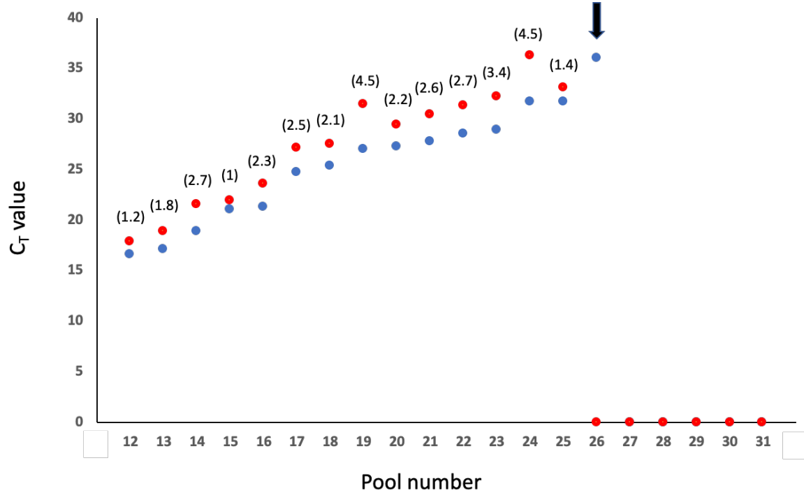
Figure 2. C_T values of amplification results of SARS-CoV-2 for pools 12-31. SARS-CoV-2 RT-PCR was done using as template nucleic acids purified from manual extraction and the C_T values obtained in the single positive samples (blue dots) and its respective pool (red dots) were graphed. Also, the change in C_T value compared with C_T value of the single positive sample present in the pool is shown in brackets. A C_T value of 0 was assigned to samples with no amplification. Pool 26 is highlighted (black arrow).
