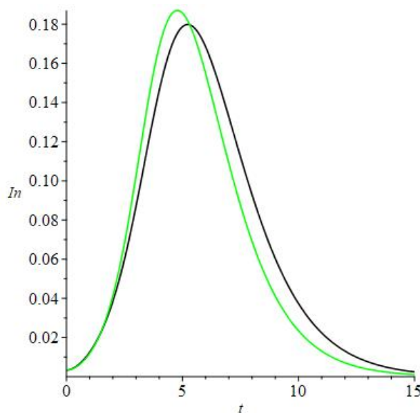
FIGURE 7. In black and green are the plots of I(t) for the simulations obtained from a_a being 0.1 and 0.2 respectively.
