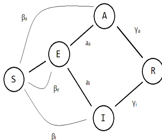
FIGURE 1. Diagram of the SEIAR model.
