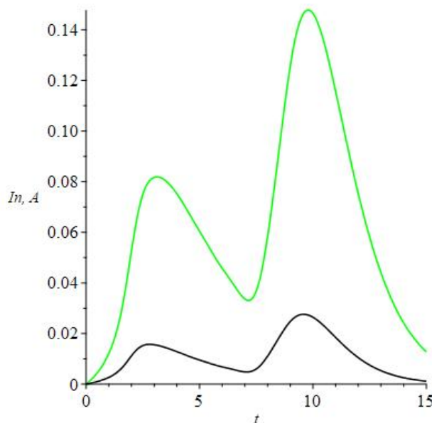
FIGURE 10. Plot of I(t) and A(t) in green and black. These represent the infected and the asymptomatic carriers respectively.
