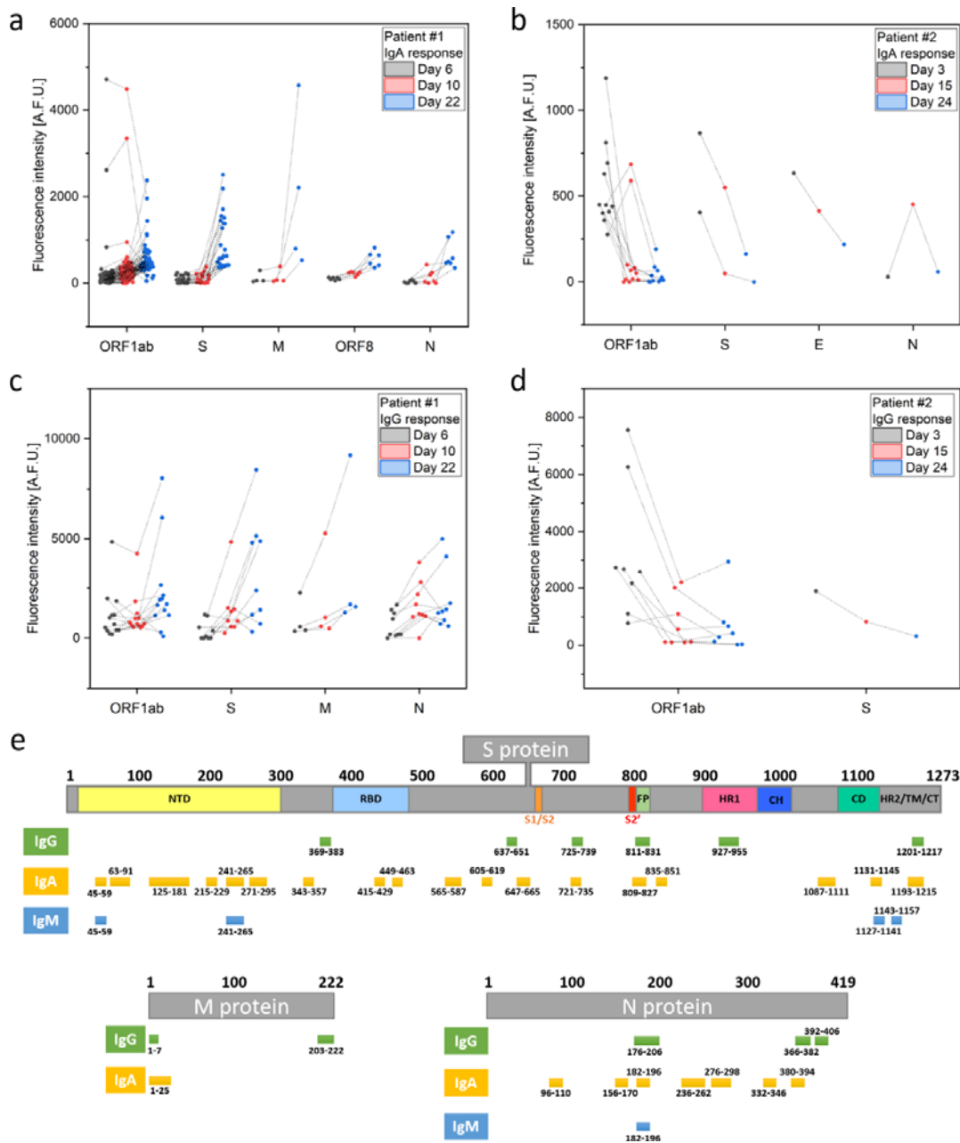
Figure 2. Reactive SARS-CoV-2 peptides following infection. (a – d) Evolution of positive responses against SARS-CoV-2 peptides at different time points after onset of disease in patients #1 (more severe symptoms) and #2 (mild symptoms). Data were generated by peptide microarray analyses, IgA (a, b) and IgG (c, d) signals are shown if at least one time point was above the 99.9 th percentile threshold of IgA/IgG signals in healthy control sample #5. Positive signals for ORF1ab polyprotein (ORF1ab), spike glycoprotein (S), envelope protein (E), membrane glycoprotein (M), ORF8 protein, and nucleocapsid phosphoprotein (N) are shown. (e) Mapping of reactive IgG, IgA, and IgM signals derived from all nine SARS-CoV-2 patient samples on the S (domains from 16 ), M, and N proteins (see Supporting Information Table S3).
