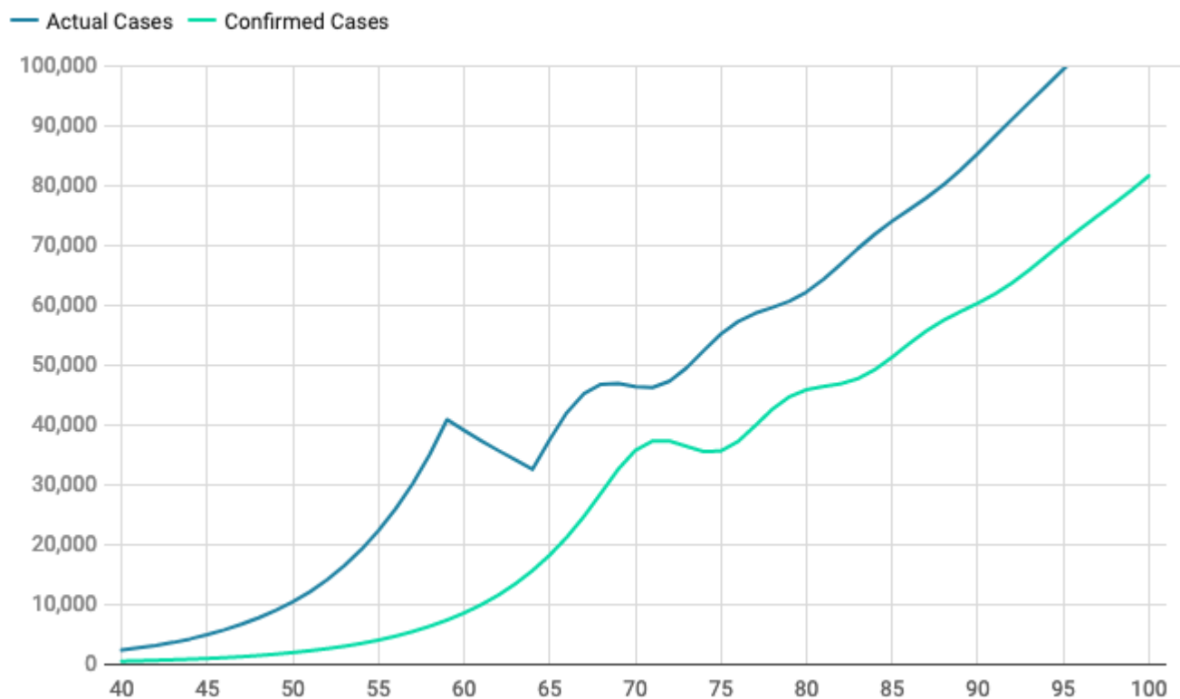
Figure 5: Predicted case and confirmation numbers after government interventions reduce R^0 from 3.5 to 1.3; adaption of measures is gradual over 6 days. The confirmed cases curve assumes that 100% of all infections are tested. This is only done to enable a direct comparison; actual test rates in most countries are significantly lower.
