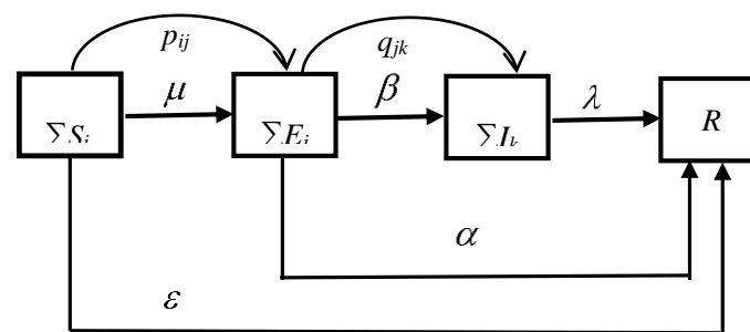
Figure II_iSEIR model Illustration
