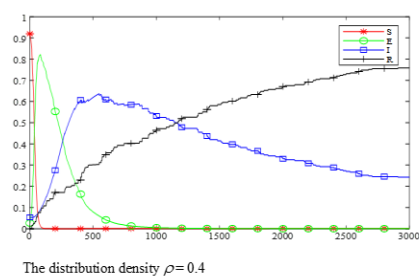
Washington State: N=0.75v million; \gamma=0.000474 (mortality rate =4.74%)
