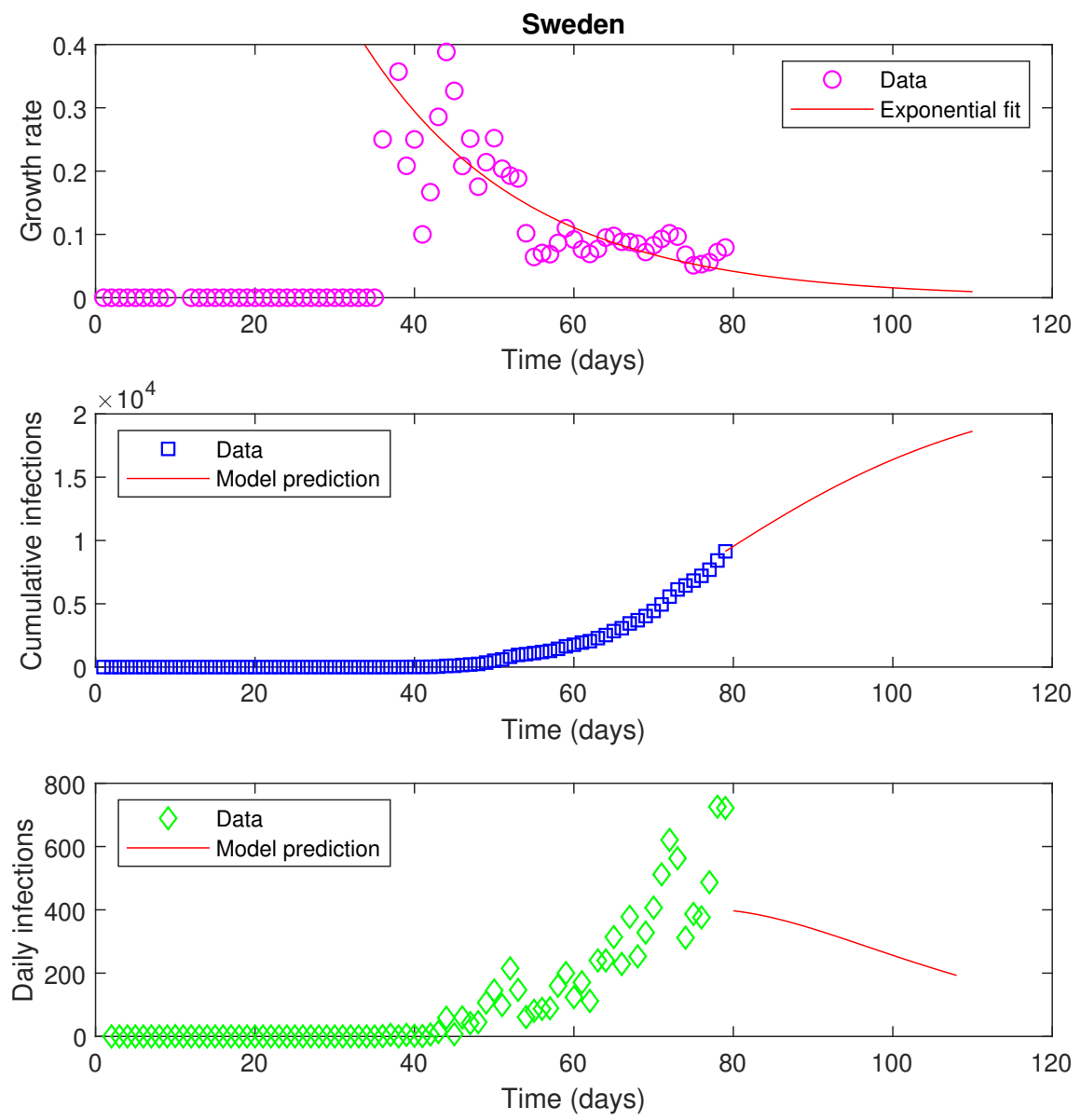
Figure 6: Data and model forecast for Sweden. Rest of caption is the same as of Fig. 3.
