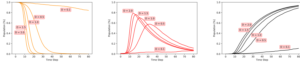
Figure 2: Effect of Population Density on S (left), I (middle), R (right) populations
