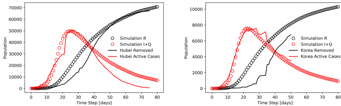
Figure 5: Random Walk Simulation fitted to data [14] from Hubei Province China and South Korea
