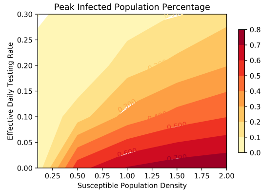
Figure 4: Peak Infection Percentage as a function of D and T
