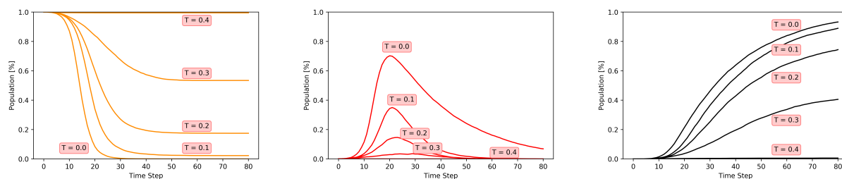
Figure 1: Effect of Testing Rate T on S (left), I (middle), R (right) populations
