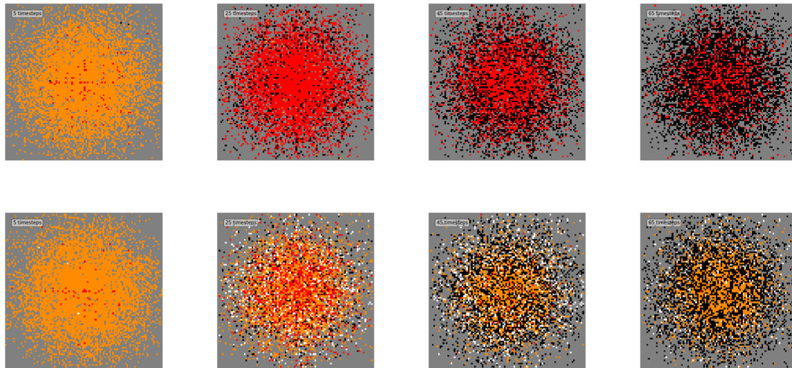
Figure 3: Visualization of effect of instituting Testing Rate T of 0.2 (bottom row), compared to no testing (top row). S denoted as yellow, I as red, R as black, Q as white. Time progression from left to right, frames taken at timesteps of [5, 25, 45, 65]
