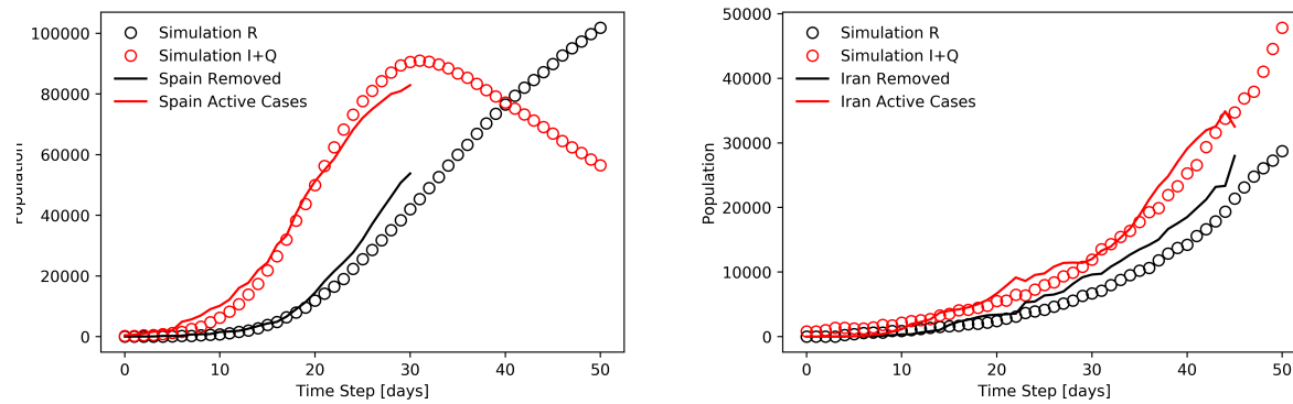
Figure 6: Random Walk Simulation fitted to data [14] from Spain and Iran
