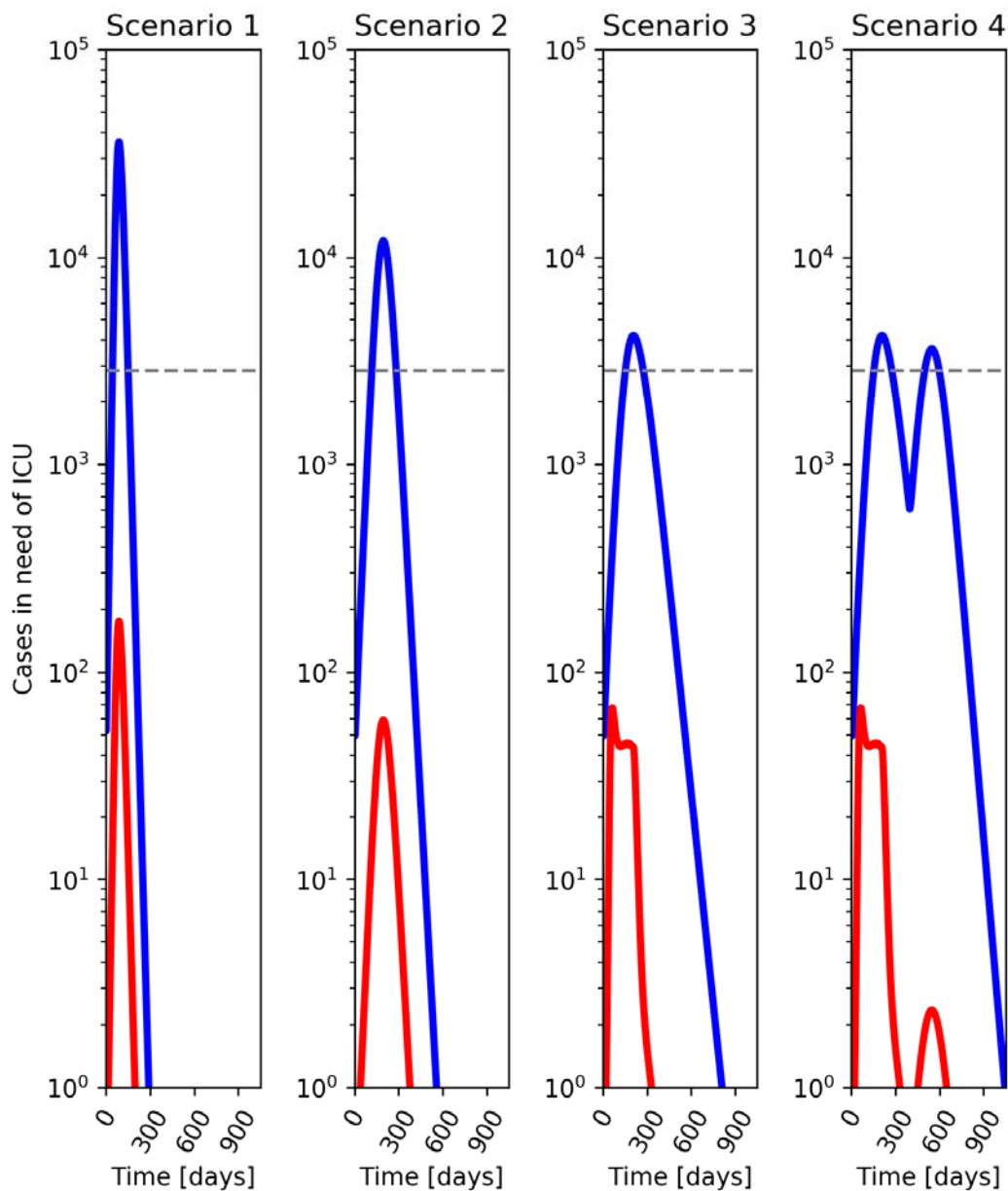
366 FIG 3. The dynamics of cases in need ICUs for four scenarios: Scenario 1- uncontrolled, 367 Scenario 2 – mitigation, Scenario 3 - controlled avalanche (CA) program, followed by 368 mitigation, Scenario 4 - CA program, followed by uncontrolled policy. The general 369 population is in blue line and those from the low-risk population is in red line.
