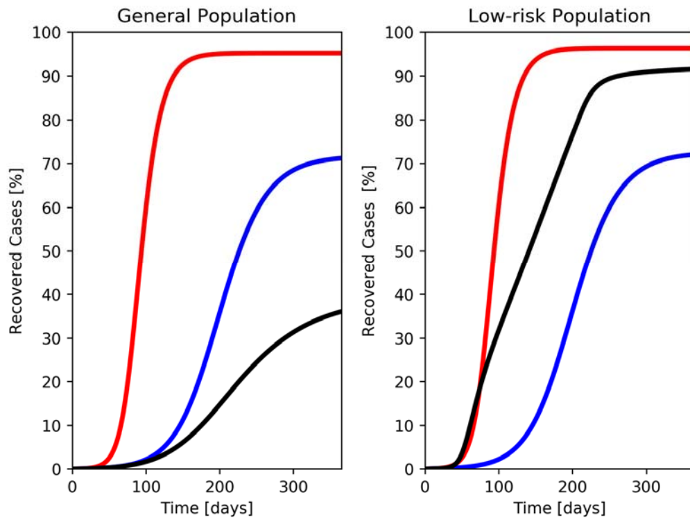
360 FIG. 2. The percentage of recovered cases in three scenarios, in red uncontrolled, in blue 361 mitigation and in black the controlled avalanche strategy. In the left side for the general 362 population and in the right side for the low risk population.
