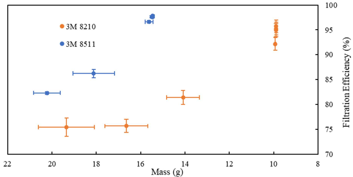
Figure 2: Filtration efficiency vs. mass for two N95 respirators made by the 3M Corporation, models 8210 and 8511. These were soaked in 70% ethanol solution, then allowed to air dry for 2.5 hours until the weight had stabilized. The original dry weights of the masks were 9.88g and 15.46g, respectively. Soaking and then air drying increased the weight of the masks to ~20.6g and ~22.8g, respectively. The masks were then pumped on and removed at intervals at specific pressures shown in Figure 3 to record the masks' mass and efficiency. As the mass of water in the mask decreased, the mask's efficiency increased along the trend indicated by the colored arrows.
