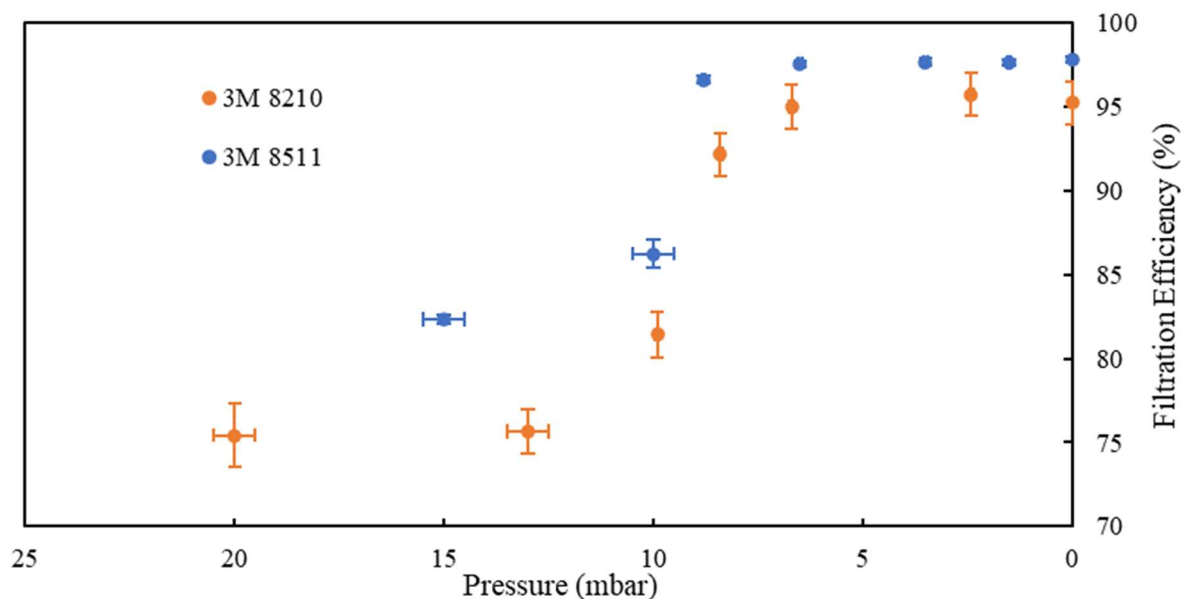
Figure 3: Filtration efficiency vs. minimum exposed pressure for two 3M N95 respirators. Filtration efficiency rapidly increases as pressure drops below ~13 mbar, corresponding with the removal of water molecules adsorbed to the surface of the microfibers. Vertical error bars are 1 standard deviation, and horizontal error bars represent measurement resolution at the given pressures. Some errors for pressures below 10 mbar are smaller than the symbol size.
