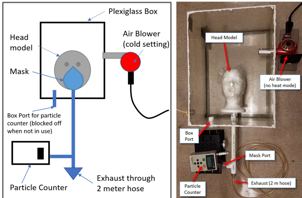
Figure 1: Left, schematic diagram of the experimental medical filter testing chamber. Right: Image of the current system with the top removed. The hand-held air blower forces ambient dirty air ( \sim 2 million particles at and above 0.3 \mu\text{m}/\text{cuf} ) into the chamber, which exits either through the mask/head plumbing system or through the background port. The ratio of the particle counts at and above 0.3 \mu\text{m} between the two ports gives a relative measure of the mask efficiency.
