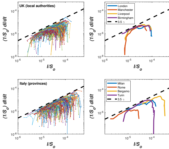
FIG. 4. Same as Figure 2 but for sample UTLAs in the UK (top left) and provinces in Italy (bottom left). Selected UTLAs and provinces are shown in the top right and bottom right panels, respectively.
