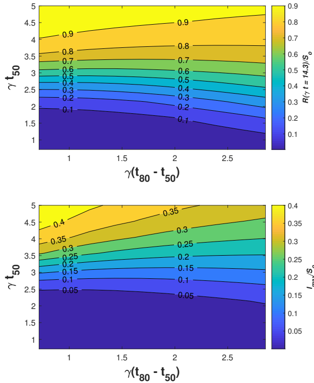
FIG. 9. Variation in cumulative number of infected relative to total population S_o (top) and in maximum number of infected relative to total population S_o (bottom) at time t with the logistic form of R_o . The R_o was set to vary from R_{o,c} = 4.5 to R_{o,u} = 1.0 . t_{50} and t_{80} are the times at which R_o is half and 80% through the the total decline.
