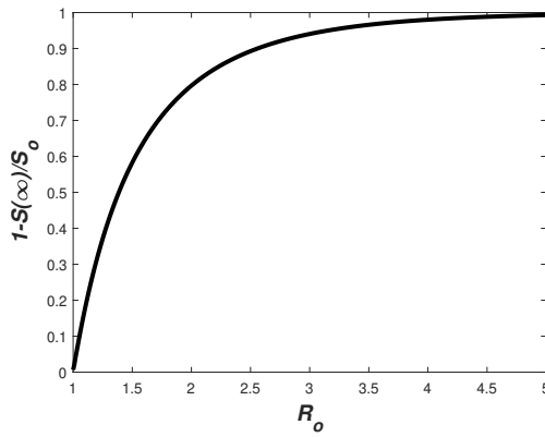
FIG. 7. Relation between total infection fraction 1 - S(\infty)/S_0 and R_0 .
