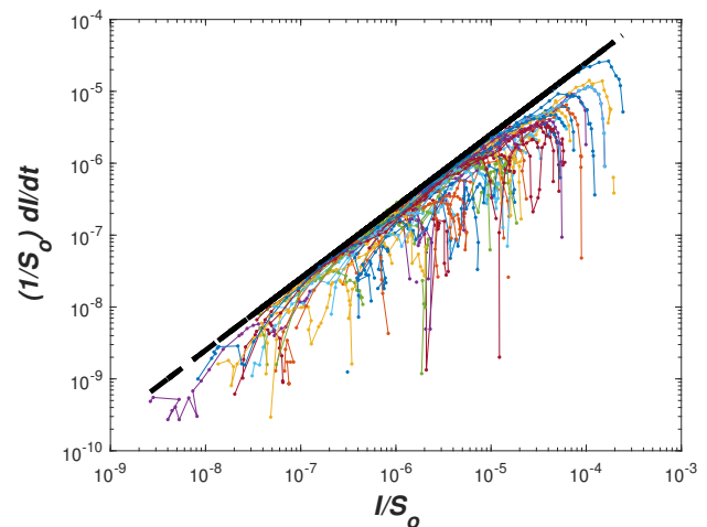
FIG. 2. Comparison between (1/S_0)(dI/dt) and I/S_0 for 57 countries. The dashed line is (R_0 - 1)\gamma , where R_0 = 4.5 , and \gamma = (1/14)d^{-1} . Negative deviations from the dashed line reflect deviations from exponential.
