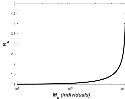
FIG. 8. Relation between total mortality and R_0 assuming \alpha_m = 0.034 and S_0 = 327M .
