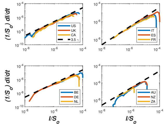
FIG. 3. Same as Figure 2 but for sample countries top left: the United States of America (US), the United Kingdom (UK), and Canada (CA); bottom left: Belgium (BE), Germany (DE), the Netherlands (NL); top right: Italy (IT), Spain (ES), and France (FR); bottom right: Australia (AU), New Zealand (NZ), and South Africa (ZA).
