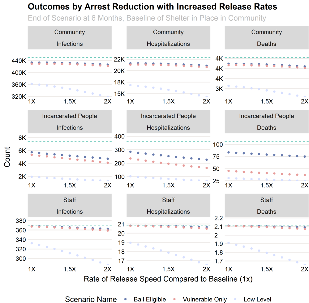
Fig 5. Cumulative infections, hospitalizations and deaths in the community (first row), among persons in jail (second row) and among jail staff (third row) for several combinations of incarceration deferment and accelerated release. Negative outcomes among persons in jail, the community as well as staff improve with faster levels of release, while the community experiences slightly worse negative outcomes.
