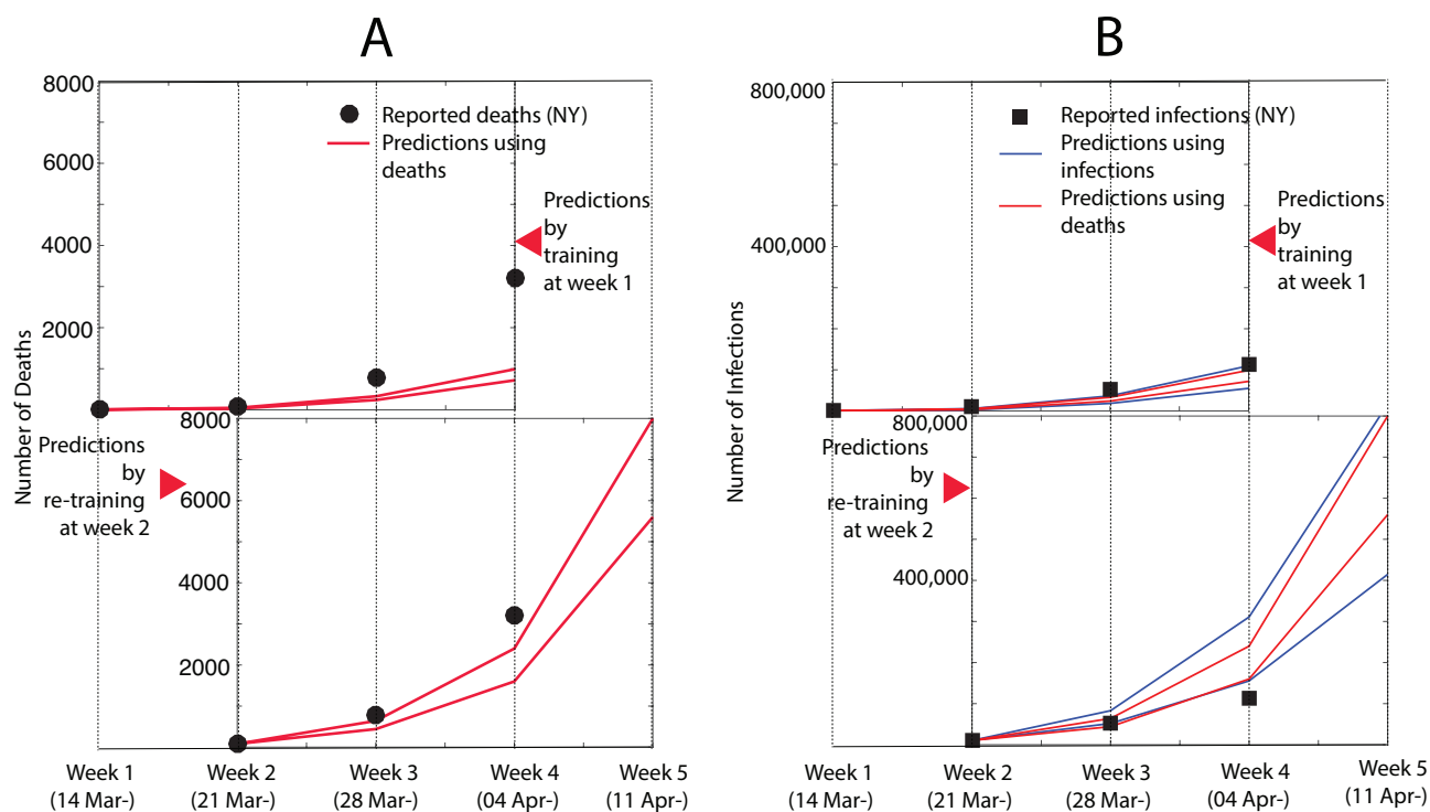
Figure 5: Adaptive predictions for New York state. The adaptive predictions were performed for the data from New York state, just as described in Figure:4.
