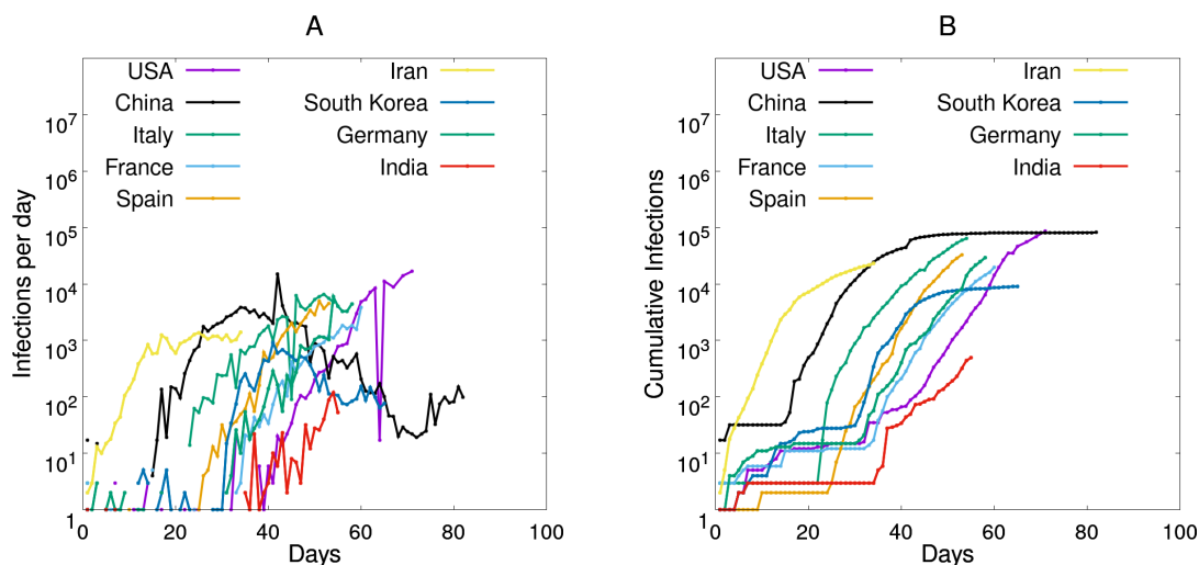
Figure 1: Time series has fluctuations. Country-wise time series data for (A) daily new infections ( dI/dt ) and (B) cumulative infections ( I ). Since the chance of infection and incubation time are stochastic, and data is recorded on a daily basis, I fluctuates. These fluctuations may be country-dependent and constrained by other factors such as the frequency of testing, specially in early days of the pandemic. To obtain a better evolution we instead focus on the ( dI/dt ) versus ( I ) which removes systematic errors
