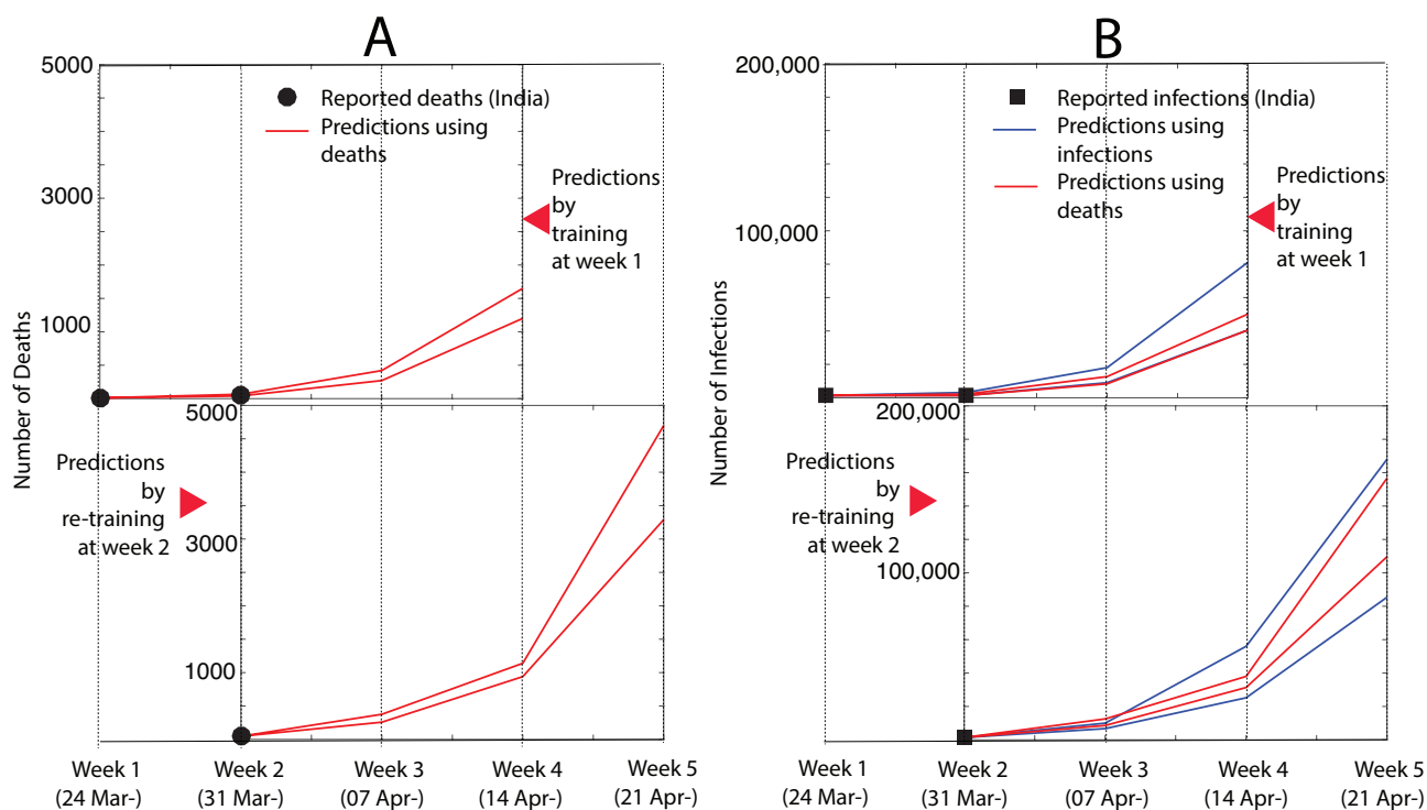
Figure 6: Adaptive predictions for India. The adaptive predictions were performed for the data from India, just as described in Figure:4 and Figure:5
