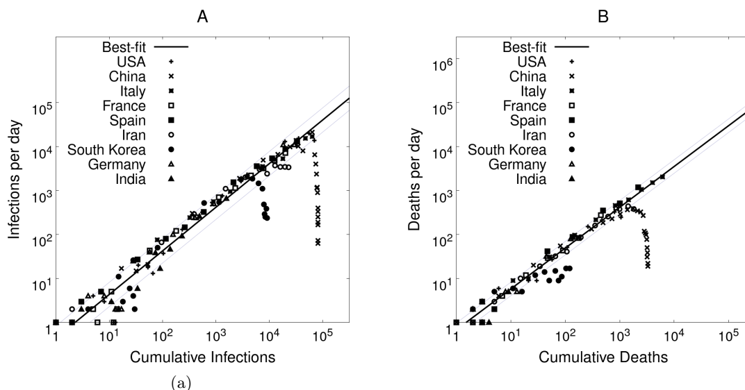
Figure 2: Universal trend in infections and deaths. The rates at which the number of infections ( I ) and number of deaths ( D ) change are explored using the COVID-19 data from many countries. (A) dI/dt versus I (B) dD/dt versus D show comparable behaviour across these countries which can be exploited in our predictions. The data from a 3-day average was used since the number of daily new infections fluctuates significantly. The standard deviation from the best fit curve in the infection plot is 0.276 and in the deaths plot is 0.153
