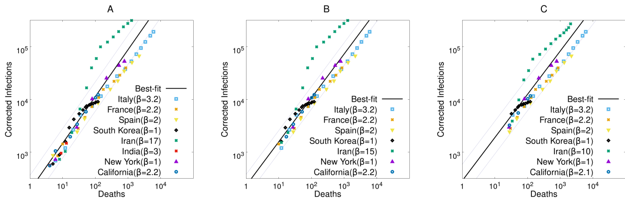
Figure 3: Using the I-D plot for estimating number of infections. These plots depict the universal relation between I and D , barring a corrective factor. This uncertainty factor that was calculated from the COVID-19 infection data of South Korea as a reference can be used for estimating infections when the number of deaths are known. \beta = \frac{\text{corrected infections}}{\text{reported infections}} was assumed to be 1 for South Korea. At any time in the evolution of the pandemic shown on this I versus D graph, using the known number of deaths in that country, the number of infections were rescaled to match with the infections in South Korea and this factor was used as \beta . The figure illustrates the procedure used for \beta when deaths are slightly lower than 10, equal to 10 and 20.
