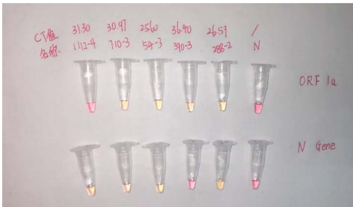
Figure 1. Comparative analysis of dual gene LAMP vs. PCR.
