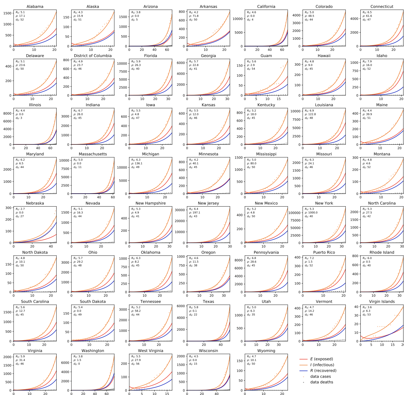
Fig. 10 COVID-19 outbreak dynamics in the United States. Reported infectious populations and simulated exposed, infectious, and recovered populations. Simulations are based on a state-specific parameter identification of the contact period B defining the basic reproduction number R_0 = C/B , and the fraction of the initial latent population \rho = E_0/I_0 for each state, for a given outbreak delay d_0 and disease specific latent and infectious periods A = 2.56 and C = 17.82 identified for the Chinese outbreak.
