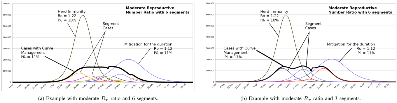
Fig. 6. Examples for moderate R_r with 6 and 3 segments showing curves for herd-, mitigated-, and controlled infections. Infection rates are limited to I_{\%om} .
