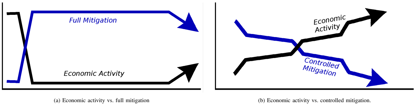
Fig. 1. Economic Health and mitigation measures are inversely proportional
