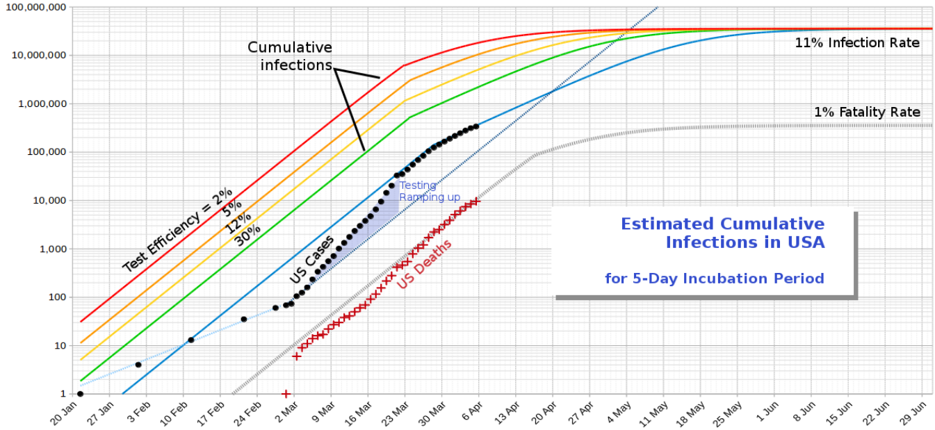
Fig. 12. An estimate of the number of infected people in the USA and a projection of COVID-19 cases.
