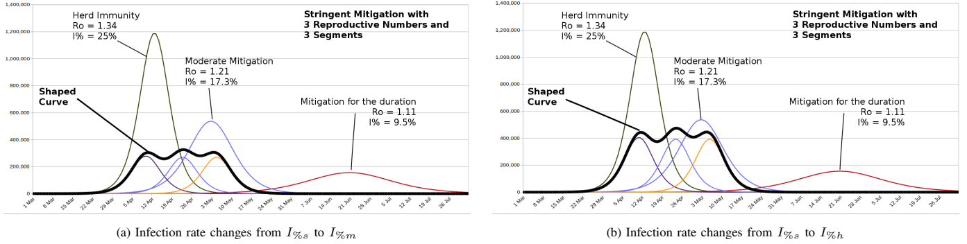
Fig. 8. Examples for stringent mitigation measures and 3 segments showing curves for herd-immunity, moderately mitigated, stringently mitigated, and controlled infections.
