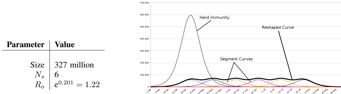
Fig. 5. An oversimplified example to illustrate the concept.
