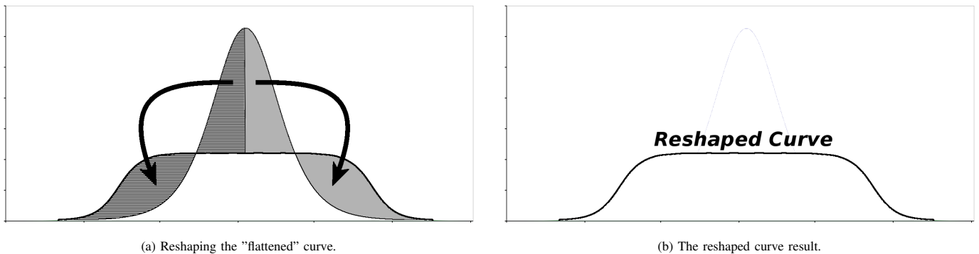
Fig. 4. The aim of the method explained graphically
