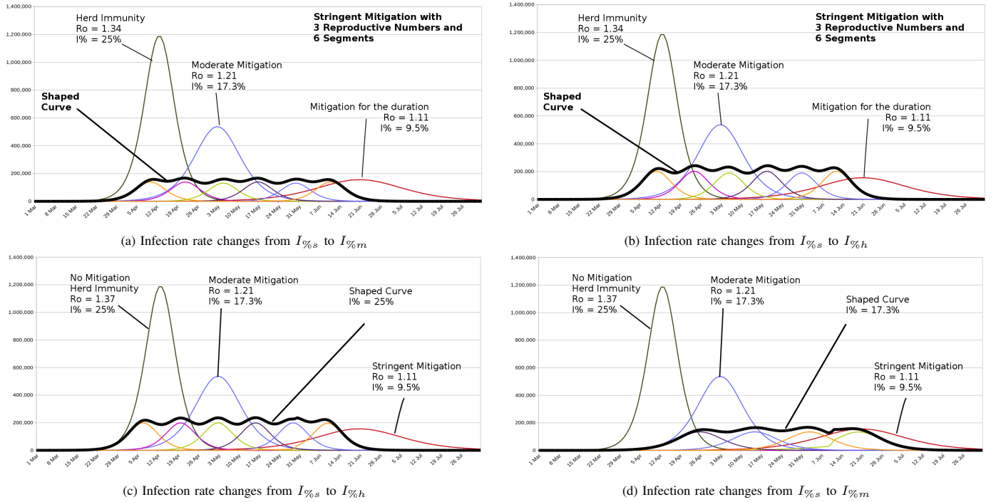
Fig. 9. Examples for various mitigation measures and up to 6 segments showing curves for herd-immunity, moderately mitigated, stringently mitigated, and controlled infections
