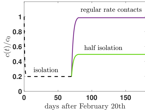
FIG. 6. Time behavior of the contact rate simulating a possible secondary event in Italy at day=70, after February 20th, when the stringent measures of isolation are hypothetically relaxed. Two scenarios are introduced, the scenario of a rapid return to the old style of life (regular rate contacts), and a more realistic scenario where only half of the regular contacts are activated.
