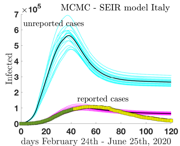
FIG. 9. (color on line) A MCMC analysis of the infected individuals (reported cases) in Italy as a function of time. The data for infected individuals of refs. [14, 15] are compared with the SEIR model predictions which include statistical uncertainties (lower curves). The green data refer to the data set used to fix the model parameters, while the yellow set spans the purely predicted period. To complete the analysis the reported cases are compared with the predictions for the class of infected non reported cases (asymptomatic) in the same period of time.
