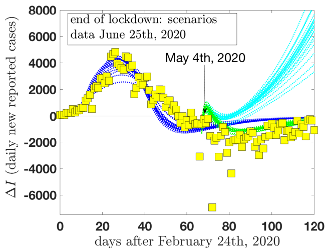
FIG. 10. (color on line) The model predictions for the daily new reported cases after February 24th, in Italy, are compared with the official data of refs. [14, 15]. In addition to the fully locked scenario (blue lines), two other scenarios are included for a mitigation of the lockdown period in Italy starting from May 4th.
