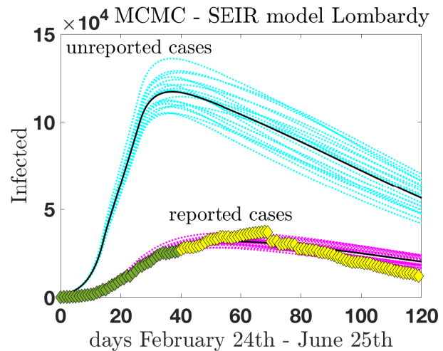
FIG. 11. (color on line) A MCMC analysis of the infected individuals (reported cases) in Lombardy y as a function of time. The data for infected individuals of refs. [14, 15] are compared with the SEIR model predictions which include statistical uncertainties (lower curves). The green data refer to the data set used to fix the model parameters, while the yellow set spans the purely predicted period. To complete the analysis the reported cases are compared with the predictions for the class of infected non reported (asymptomatic) cases in the same period of time.
