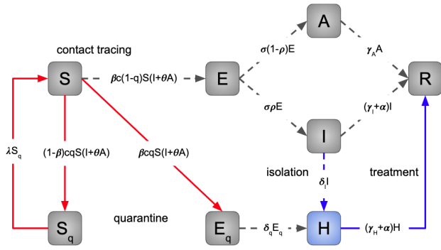
FIG. 1. Diagram of the model simulating the novel Coronavirus (Sars-CoV-2) infection in Italy. The population is stratified in Susceptible ( S ), exposed ( E ), asymptomatic infected individuals ( A ), infectious with symptoms ( I ), hospitalized ( H ) and recovered ( R ), quarantined susceptible ( S_q ), isolated exposed ( E_q ) compartments. Interventions like intensive contact tracing followed by quarantine and isolation are indicated (cfr. ref. [8]).
