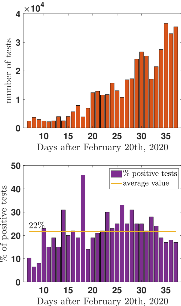
FIG. 3. (color on line) upper panel: The per-day number of tests performed in Italy in the last weeks. lower panel: Percentage of positive test per day. The average value is also shown (continuous horizontal line). Data from refs. [14, 15].
