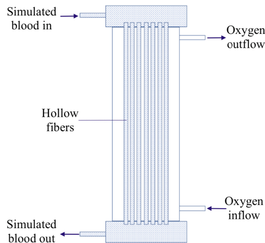
Fig. 1. Schematic of the experimental set up showing oxygen passed through the dialyser via the dialysate inlet while deoxygenated water was passed through the hollow fibres in counter-current to the oxygen
