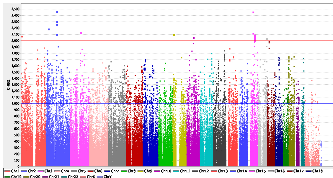
Fig.1: Manhattan Plot. GWAS with 753 European genomes were compared to 838 Eastern Asian genomes. Out of 597,573 SNPs employed, 385,450 (64.5%) markers revealed highly significant variation between Europeans and East Asians. The chi square values are plotted in Y-axis. The SNPs are designated with dots. The SNPs with chi square values >1000 are indicated with the blue line and those with chi square value >2000 are indicated with the red line. While 18 SNPs showed chi square values >2000, 2,992 SNPs had chi square values >1000.
