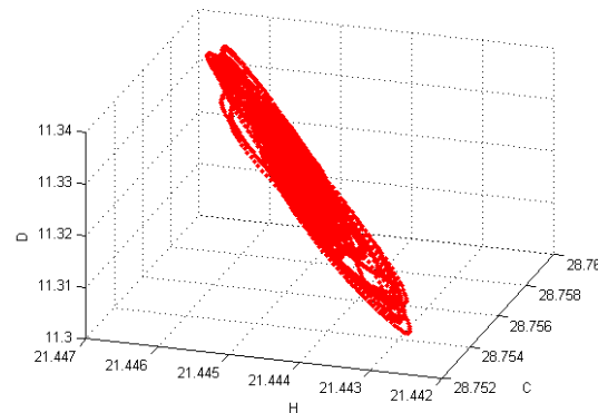
Figure 8 Scatter diagram for COVID-19 outbreak
