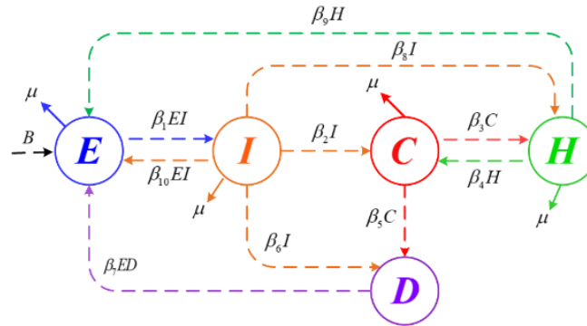
Figure 1 Transmission dynamics of COVID-19
