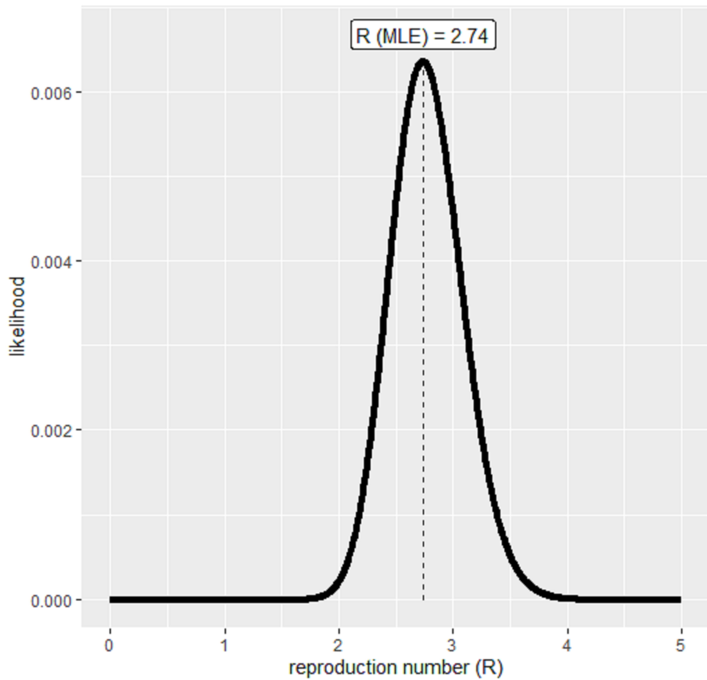
Likelihood distribution of R
