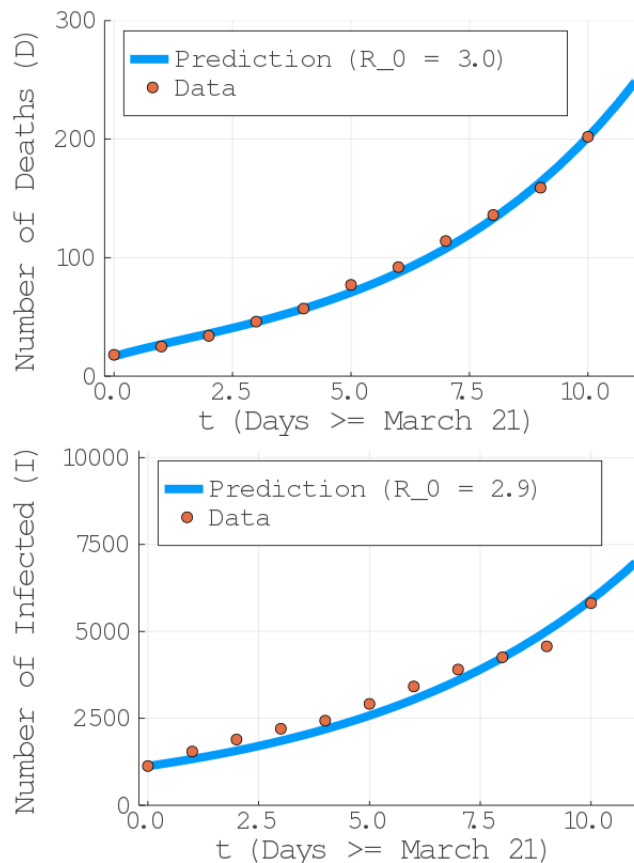
FIG. 2. Estimation of the parameter R_0 by means of data fitting for: (top) the evolution of the number of deaths (D) and (bottom) number of infected persons (I).
