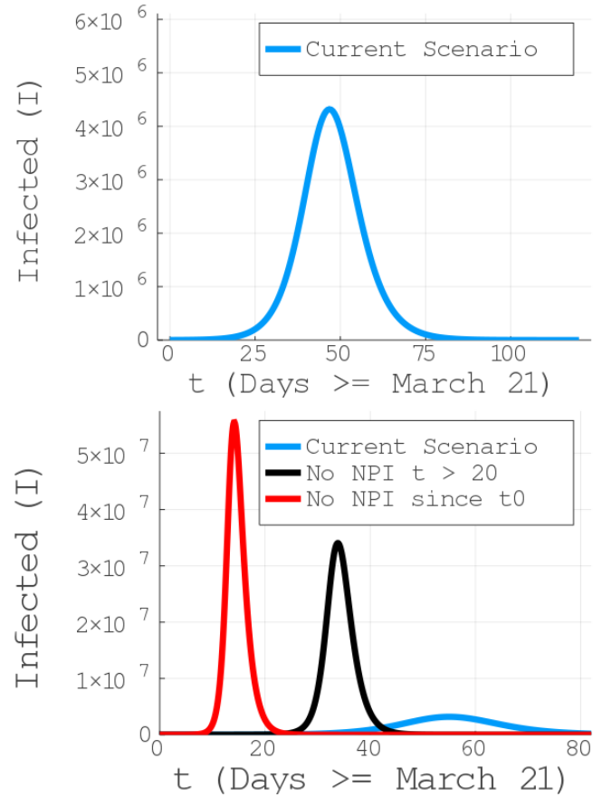
FIG. 3. Infected individuals as a function of time for the current NPI measures being taken in Brazil. The current measures not only have reduced the number of infections but also moved the peak of the contamination to later date, given the authorities the necessary time for preparation. The model has a prognostics of million of infected persons in the current scenario and tens of millions in the case of returning to a zero NPI scenario, if adopted 20 days after t_0 (March, 21), meaning t_{NPI} = April, 11. Notice a current relatively slow progress, until 30 days from March, 21 (April, 21). Stricter control measures, such as an intense quarantine, are more effective within this window.
