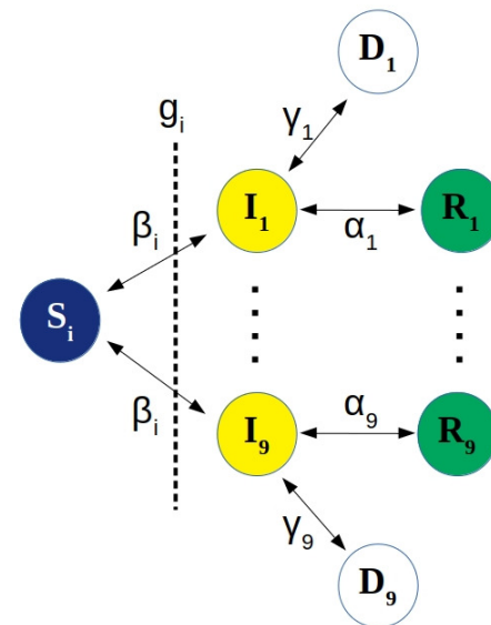
FIG. 1. Schematic representation of the SIRD model under a NPI policy g_i . The individuals can flow among four states in each of the age group i : susceptible ( S_i ) to infected ( I_i ) with rate \beta_i , who can recover ( R_i ) at a rate \alpha_i or die ( D_i ) at a rate \gamma_i , the recovered populations do not become susceptible, as is suggested for COVID-19 [12]. The NPIs policies serve as a barrier to contain the infection. The quantity (g_i S_i) represents the fraction of people not respecting the NPI policy, therefore still susceptible.
