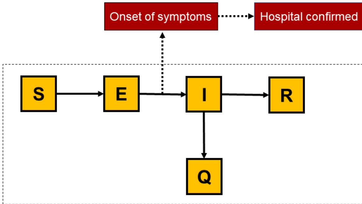
Figure 2: SEIQR model structure. The population was divided into five compartments: S (susceptible), E (exposed and partly asymptotically infectious), I (symptomatically infectious), Q (quarantined), and R (recovered). A fraction of symptomatic infections were confirmed and documented by hospitals.
