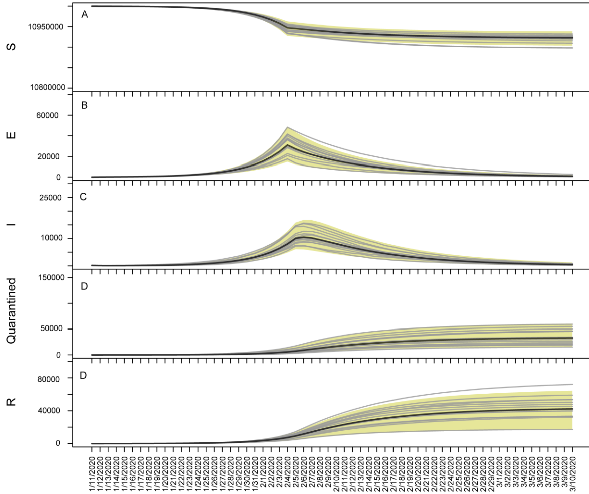
Figure S2. Prediction of the cumulative number of individuals in S (susceptible), E (exposed and partly asymptotically infectious), I (symptomatically infectious), Q (quarantined), and R (recovered) statuses separately.
