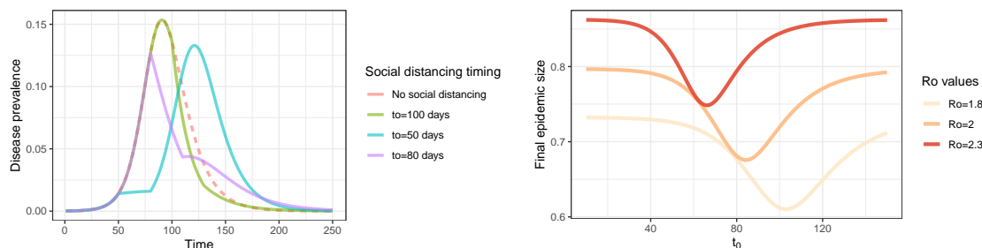
Figure 2: (left) Disease prevalence for different t_0 values and no social distancing (dashed line) with R_0 = 2 . (right) Final epidemic size for different values of t_0 for three different values of R_0 . For all simulations, \gamma = 1/10 , T = 30 days, r = 0.55 , I(0) = 0.01\% .
