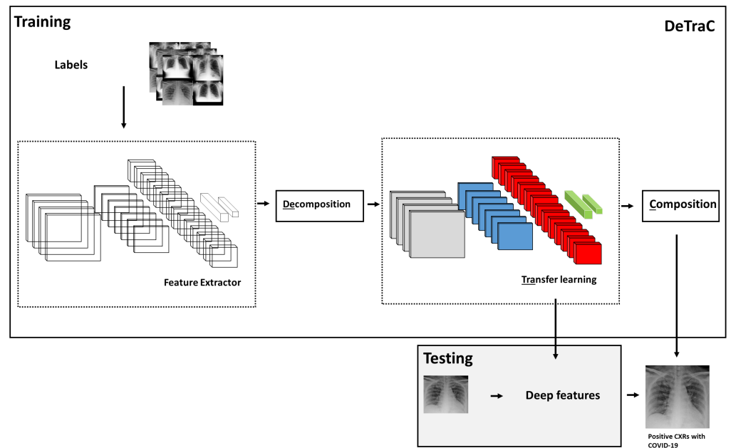
Fig 2. Decompose , Transfer , and Compose ( DeTraC ) model for the detection of COVID-19 from chest X-ray images.
