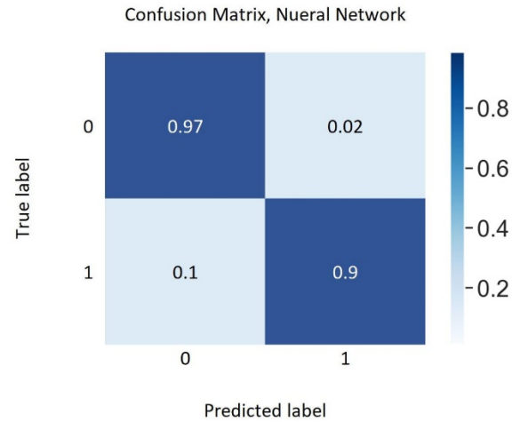
Figure 5. Neural Network confusion matrix
