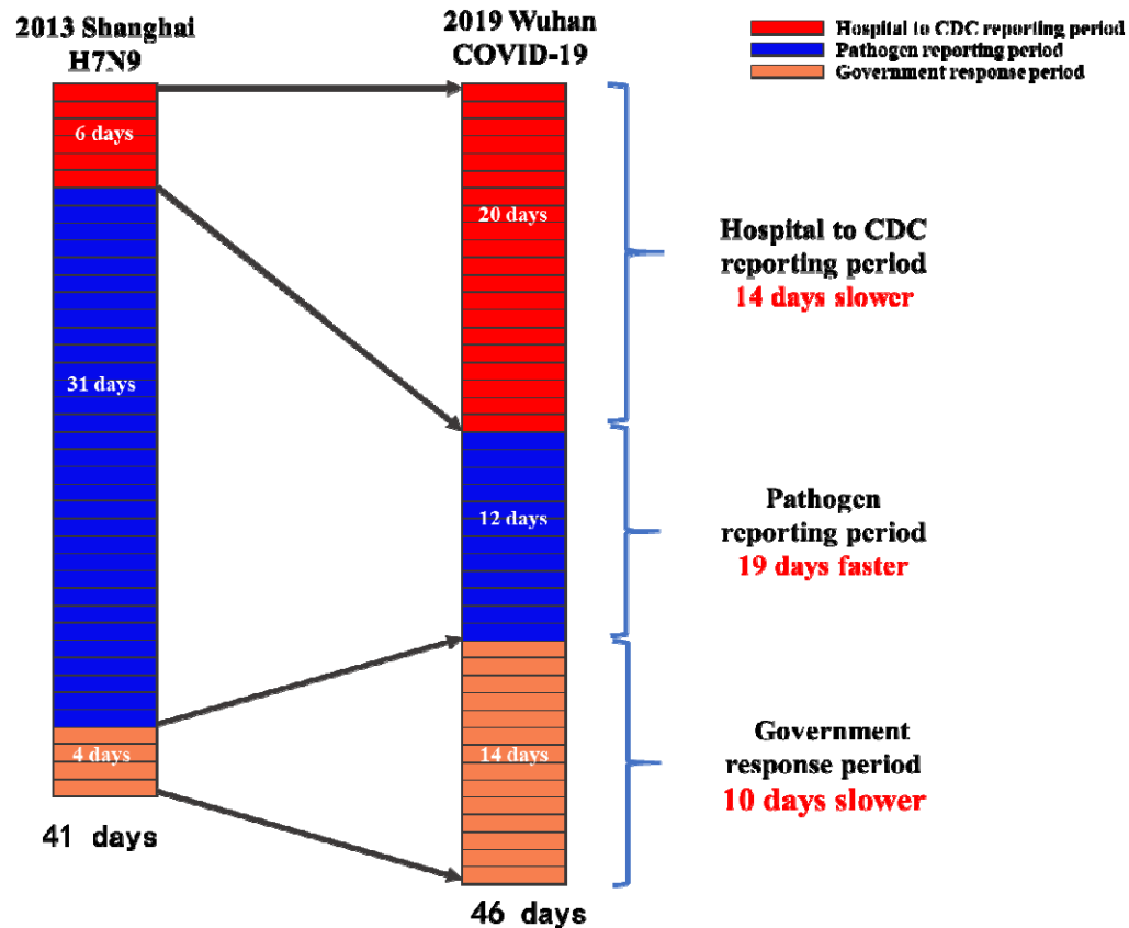
204 Figure 2. Comparison of three critical emergency disposal speed between H7N9 avian influenza (2013) in Shanghai versus coronavirus 205 disease 2019 in Wuhan.
