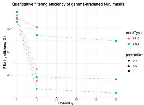
Fig. 2. Filtering efficiency
