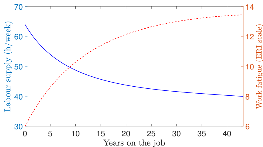
Figure 3: Hours and fatigue profiles over time converge to their steady-state values
