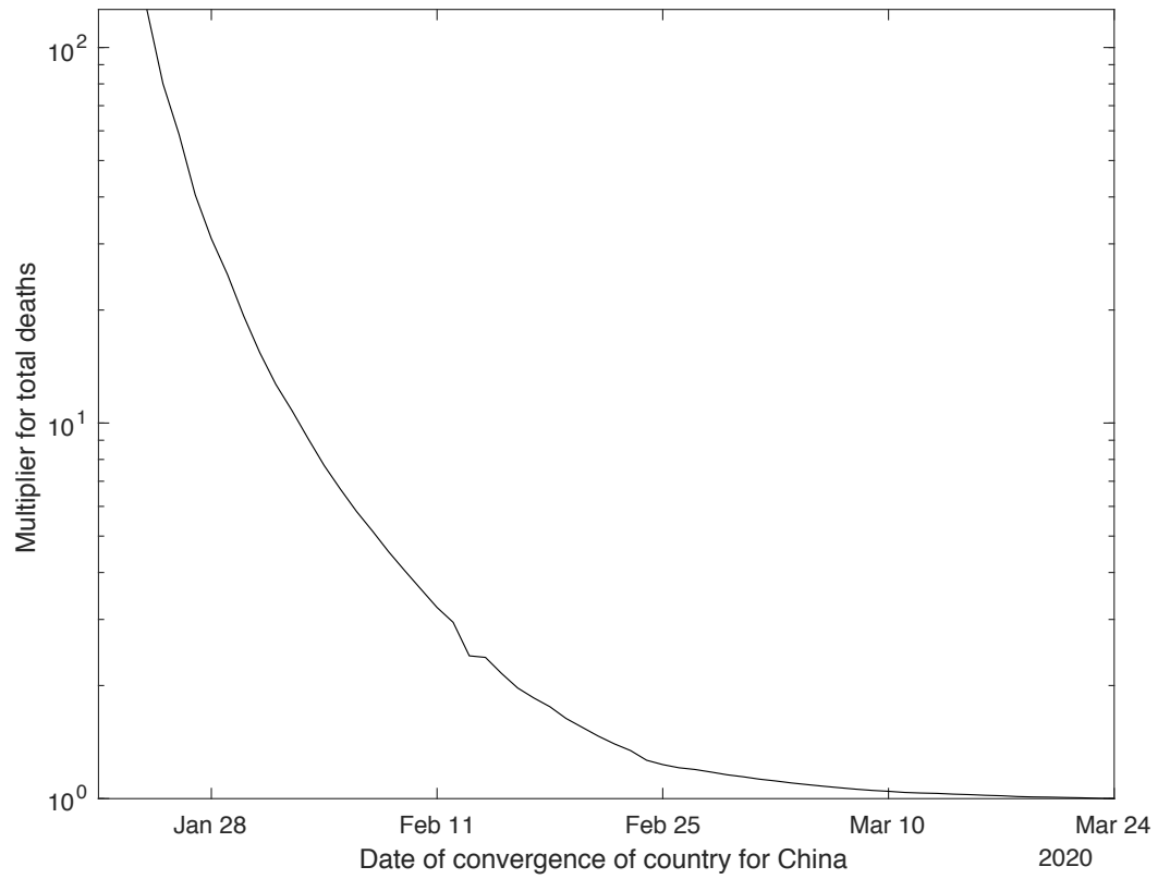
Figure 2: Multiplier for current total deaths for a country outside China to give the final total deaths, plotted as a function of the date of convergence for the Chinese dataset.
