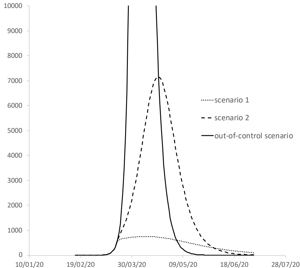
Figure 4. Graphical representation of the different scenarios considered in this study.
