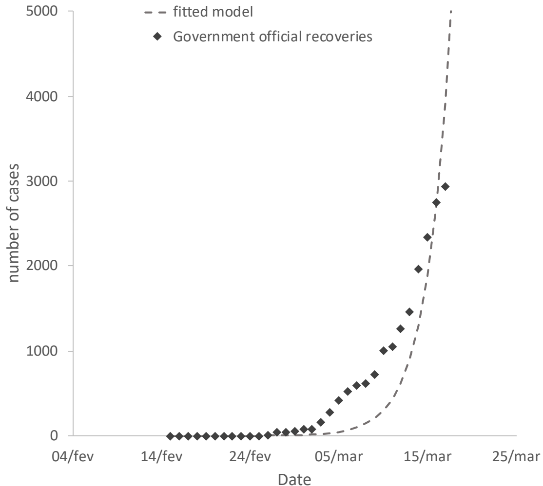
Figure 2. Graphical representation of the fitted model to the Italian government official recoveries.
