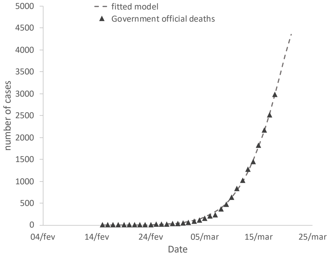
Figure 1. Graphical representation of the fitted model to the Italian government official death toll.
