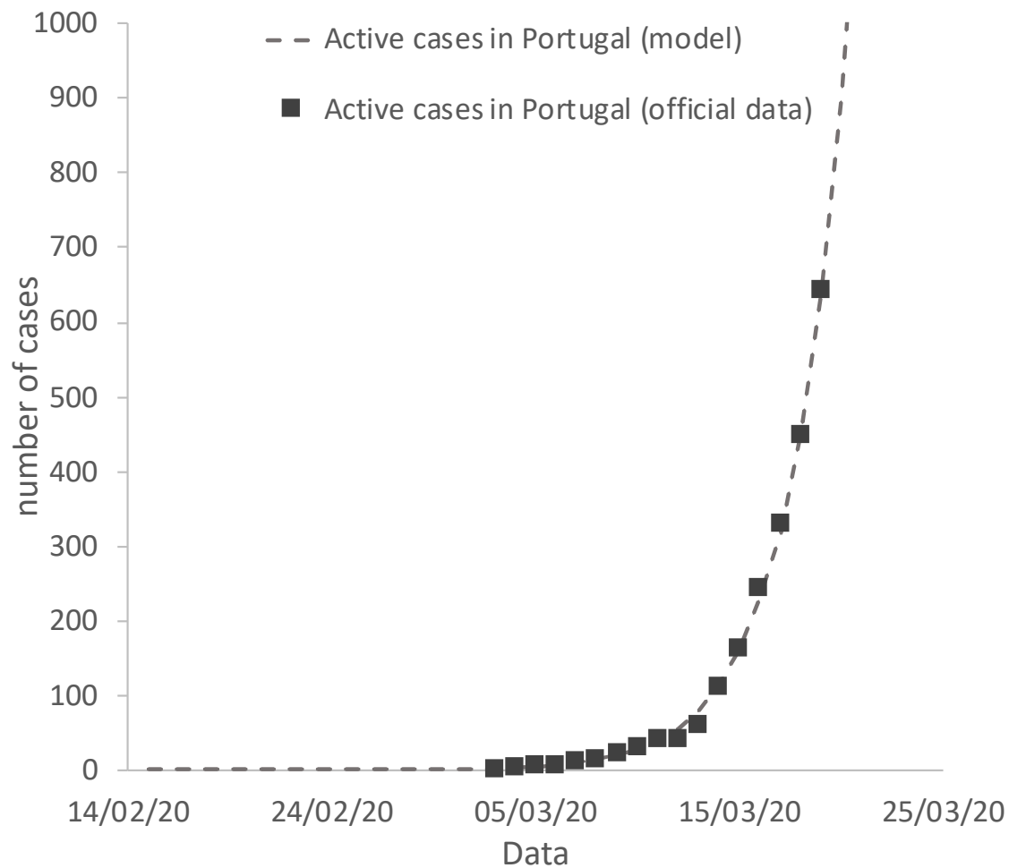
Figure 3. Graphical representation of the fitted model to the Portuguese government official active cases.
