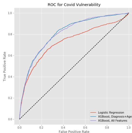
Figure 1: A Receiver Operating Characteristic graph depicting the performance of the three models.
