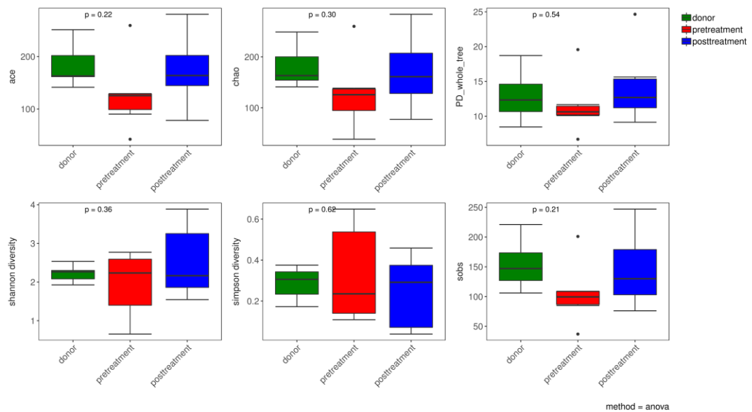
Figure 4 Alpha diversity index box chart The abscissa represents sample grouping and the ordinate was alpha index, healthy donors, active UC patients (marked as pretreatment) and post FMT treatment (marked as post-treatment) showed no significant difference ( p > 0.05 ).
