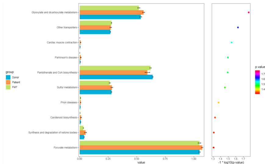
Figure 9 PICRUSt predicted the distribution of KEGG secondary metabolic pathways.
