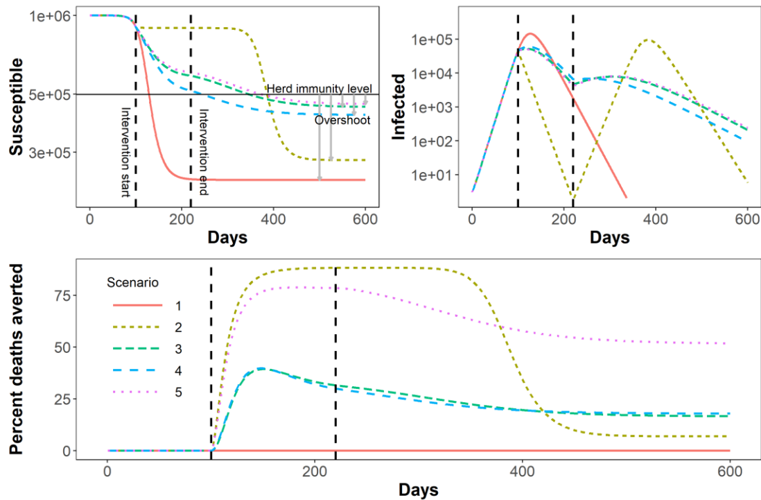
Figure 1: Susceptible, Infected, and percent deaths averted for different intervention scenarios. Scenario S1 shows a situation without any interventions, the maximum number of people get infected, the overshoot (gray arrow) is large, susceptibles drop far below the herd immunity level (solid horizontal line). In S2, strong interventions are applied to all groups, elderly are fully protected and children and adults have a reduction in infection rates of 90%. This is enough to drive down the outbreak while the interventions are active, thus initially reducing mortality the most. However, once the interventions are stopped, a consecutive outbreak occurs, leading to an overshoot and drop in susceptibles similar to the first scenario, and the overall number of averted deaths at the end of the outbreak is low. In S3-S5, the
