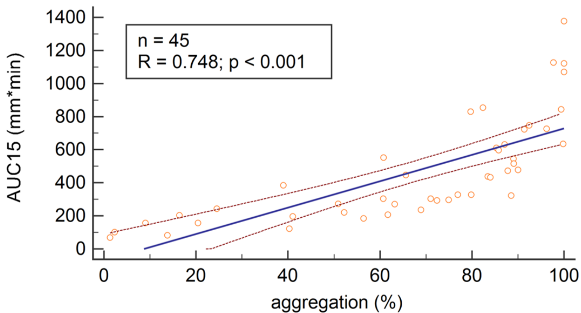
Figure 2 Bivariate scatter plot of percentage of platelet aggregation against AUC15 ( n = 45 , R = 0.748 , 95% CI = [0.582, 0.854], p < 0.001 ). Solid blue line = linear regression line, dashed red lines = 95% CI.
