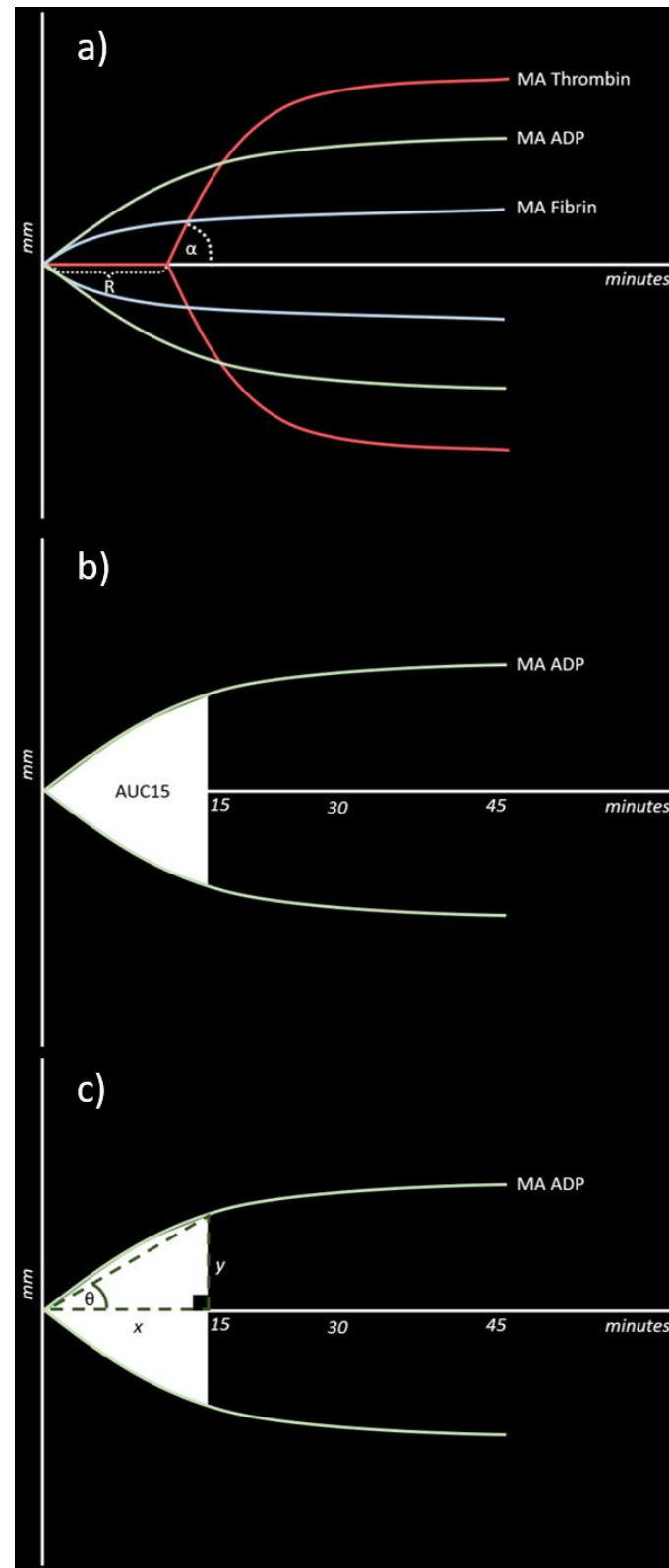
Figure 1 (a) An example TEG 6s tracing following a Platelet Mapping™ assay. MA = maximum amplitude, \alpha angle = angle of thrombin curve between 2-20mm amplitude, R time = latency time between start of test until 2mm amplitude on the thrombin curve is achieved. (b) Exact area under the curve at 15 minutes that can only be calculated using specialised computer software. (c) Right-angled triangle overlaid on AUC15 to approximate AUC15. \theta angle = an approximation of the equivalent of the \alpha angle for the ADP curve, x = 15 minutes, y = ADP curve amplitude at 15 minutes.
