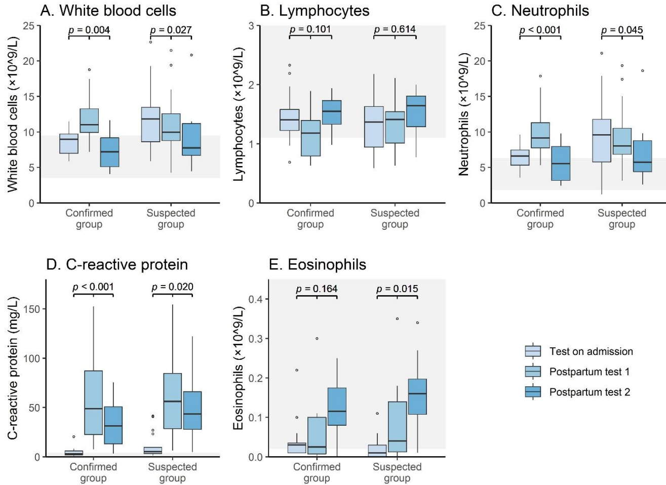
Figure 1. Box plots of blood test results of the confirmed and suspected case groups. Reference ranges of blood tests results are highlighted in grey. P values were calculated from Friedman tests for difference of blood tests results across three tests.
