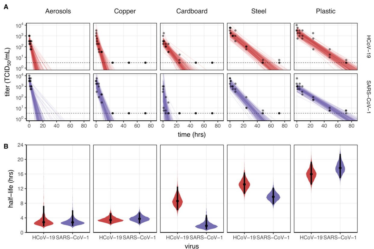
239 240 Figure 2. Estimated exponential decay rates and corresponding half-lives for HCoV-19 and SARS-CoV- 241 1. Experimental conditions are ordered by posterior median half-life for HCoV-19. A: Regression plots 242 showing predicted decay of virus titer over time; titer plotted on a logarithmic scale. Points show 243 measured titers and are slightly jittered along the time axis to avoid overplotting. Lines are random draws 244 from the joint posterior distribution of the exponential decay rate (negative of the slope) and intercept 245 (initial virus titer), thus visualizing the range of possible decay patterns for each experimental condition.
