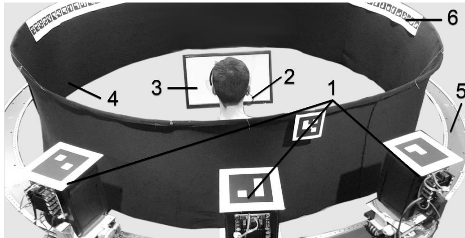
Figure 1: The robotic measurement setup during the minimum audible angle (MAA) assessments at 180-degree azimuth. Three wireless controllable audio robots with optical tracking markers (1), eye-tracking glasses (2), a touch screen with a graphical user interface (GUI) (3), sound-transparent curtain (4), a low-noise rail (5) and azimuth reference markers (6).
