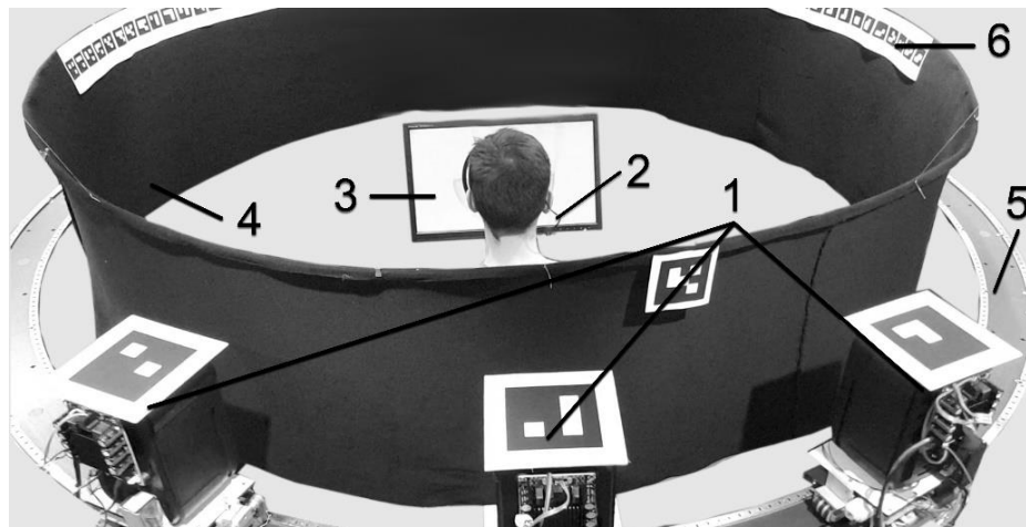
471 Figure 1: The robotic measurement setup during the minimum audible angle (MAA) assessments at 472 180-degree azimuth. Three wireless controllable audio robots with optical tracking markers (1), eye- 473 tracking glasses (2), a touch screen with a graphical user interface (GUI) (3), sound-transparent 474 curtain (4), a low-noise rail (5) and azimuth reference markers (6).
