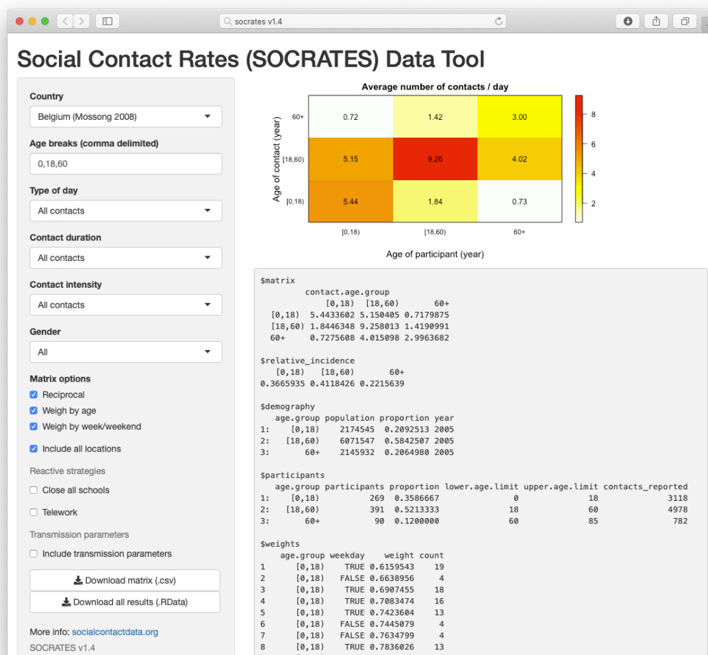
Figure 1: Screenshot of the online SOCRATES application [37]. The user interface enables the selection of country data in combination with temporal and contact features. The social contact matrix is shown on the right in addition to principal results and statistics. When users include reactive measures such as school closure and/or increased teleworking, the R_0 ratio is added to the output (not shown).
